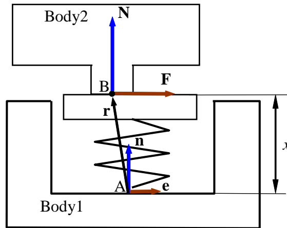
Figure 1.266. Scheme of the force element
