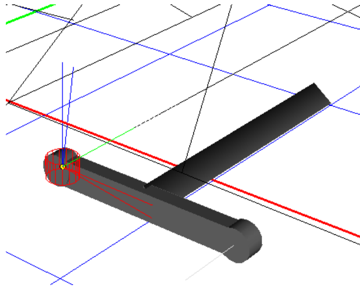
Figure 1.262. Example of a bushing: model of a car VAZ21_09 from directory Samples/Automotive
