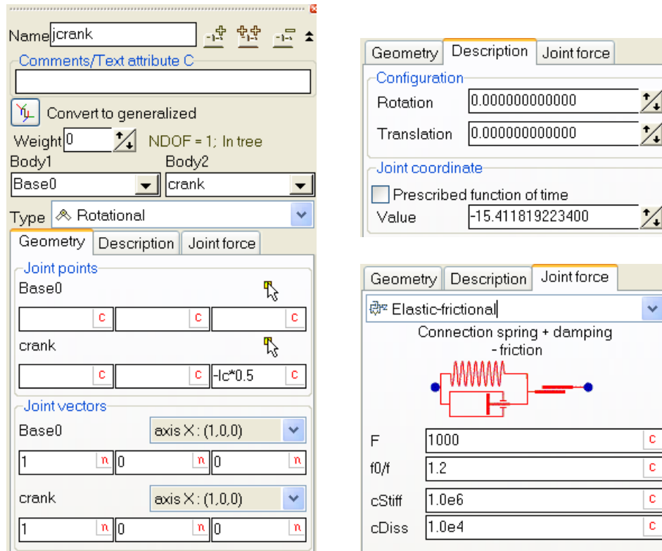
Figure 1.179. Parameters of a rotational joint
