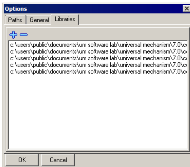
Figure 1.9. Component libraries
