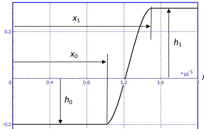
Figure 1.35. Step function
