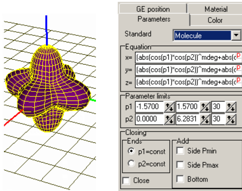
Figure 1.110. Parametrical GE
