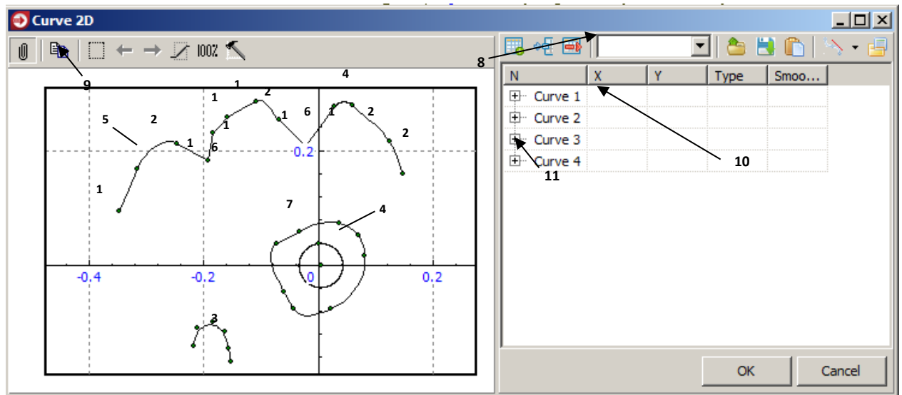
Figure 1.134. Curve editor
