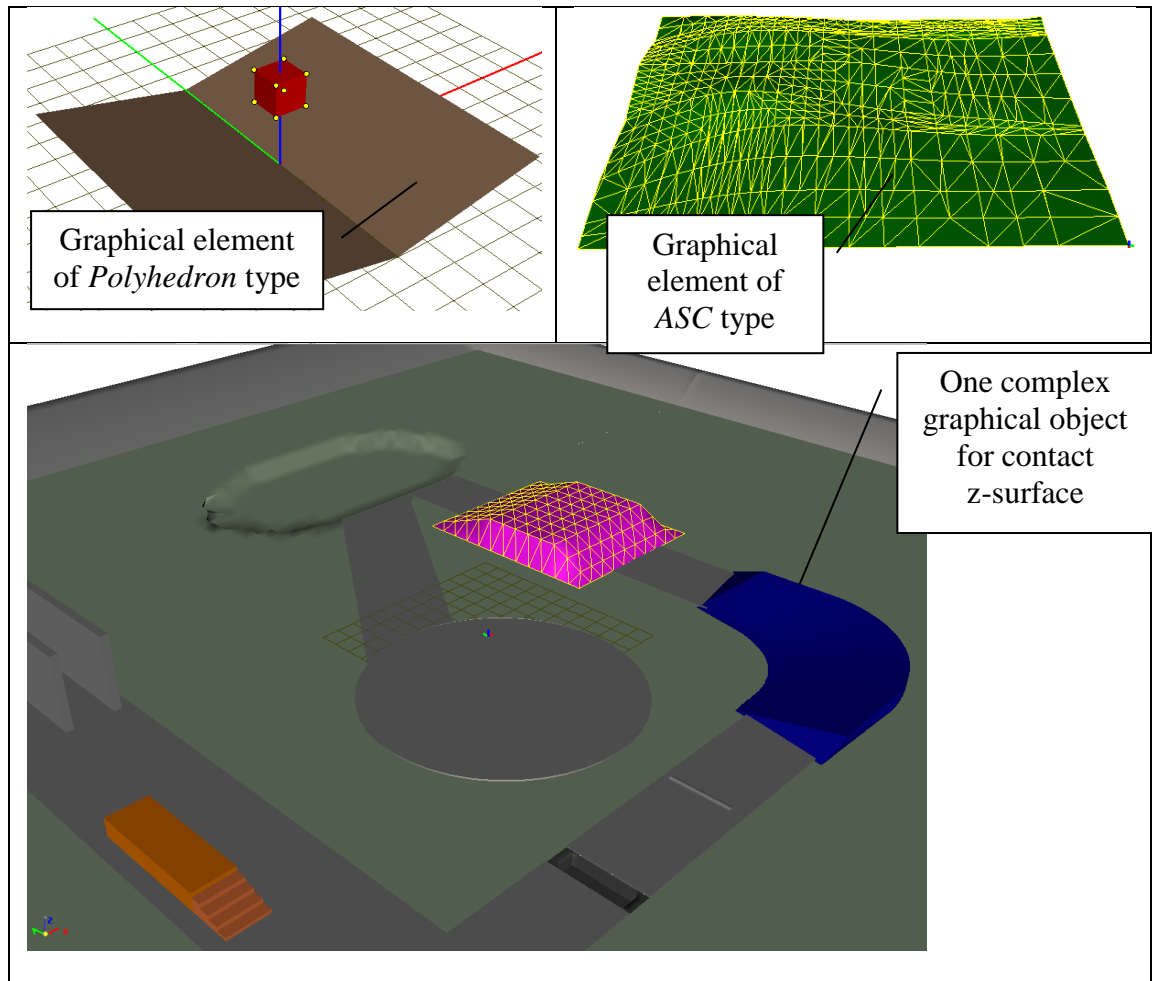
Figure 1.250. Examples of graphical objects for z-surface
