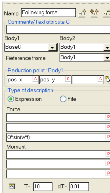
Figure 1.251. Example of a harmonic following force
