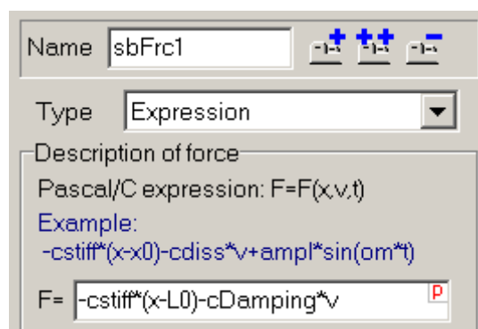
Figure 1.225. Example of a list of two forces
