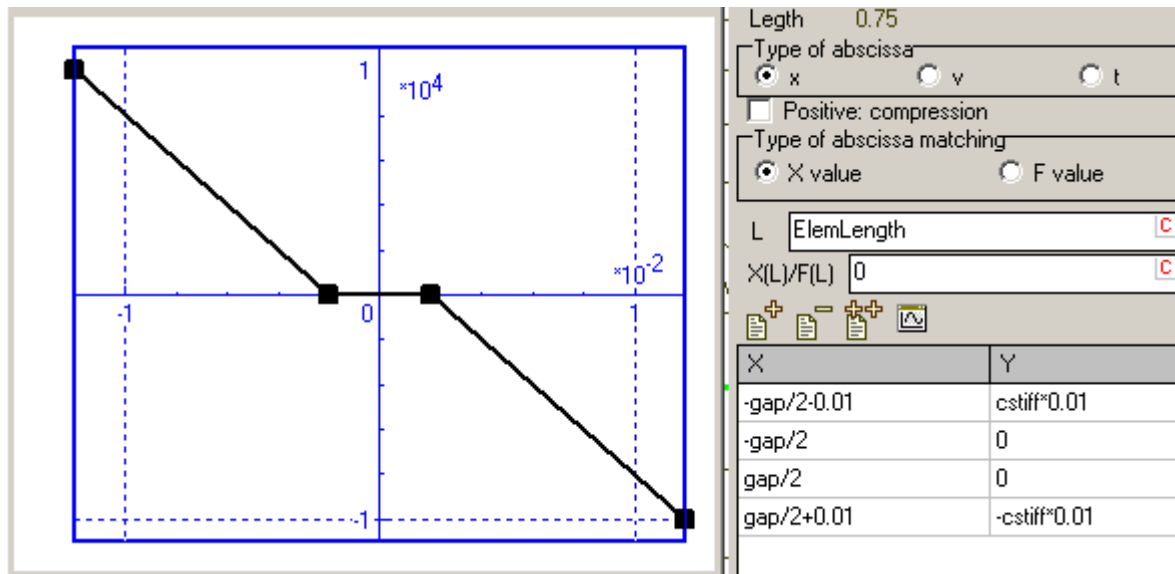
Figure 1.213. Elastic bipolar force element with a gap, which value is set by the gap identifier
