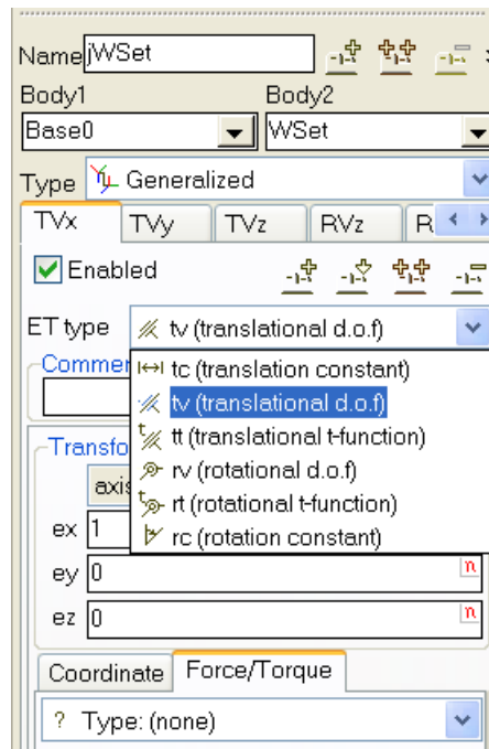
Figure 1.184. Generalized joint
