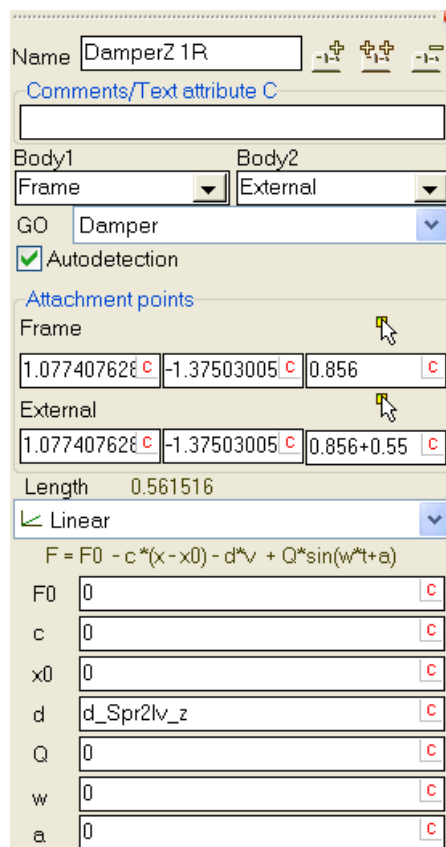
Figure 1.226. Bipolar force element
