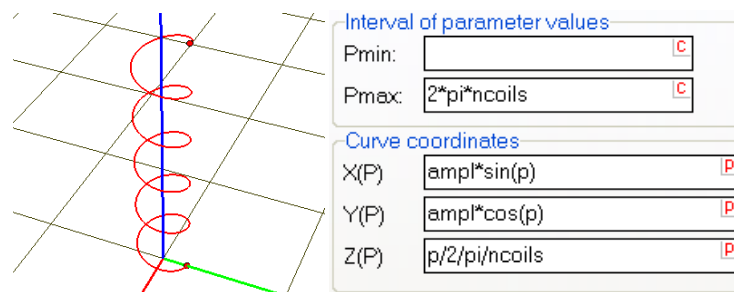
Figure 1.93. Analytical description of a spiral with parameterized number of coils
