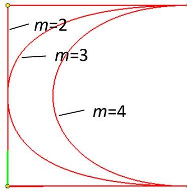
Figure 1.98. Open B-splines of different order for the same set of points
