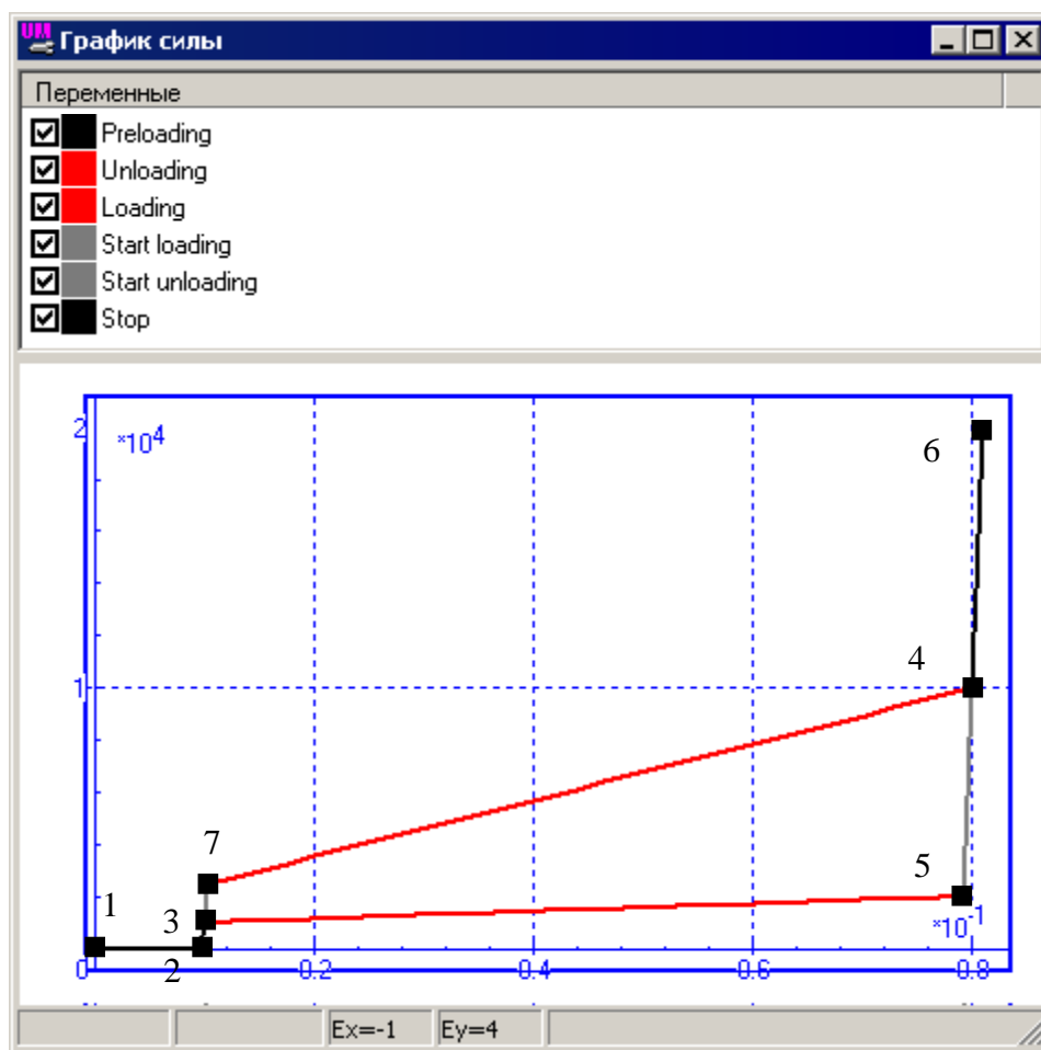
Figure 1.221. Graphic window with hysteresis data
