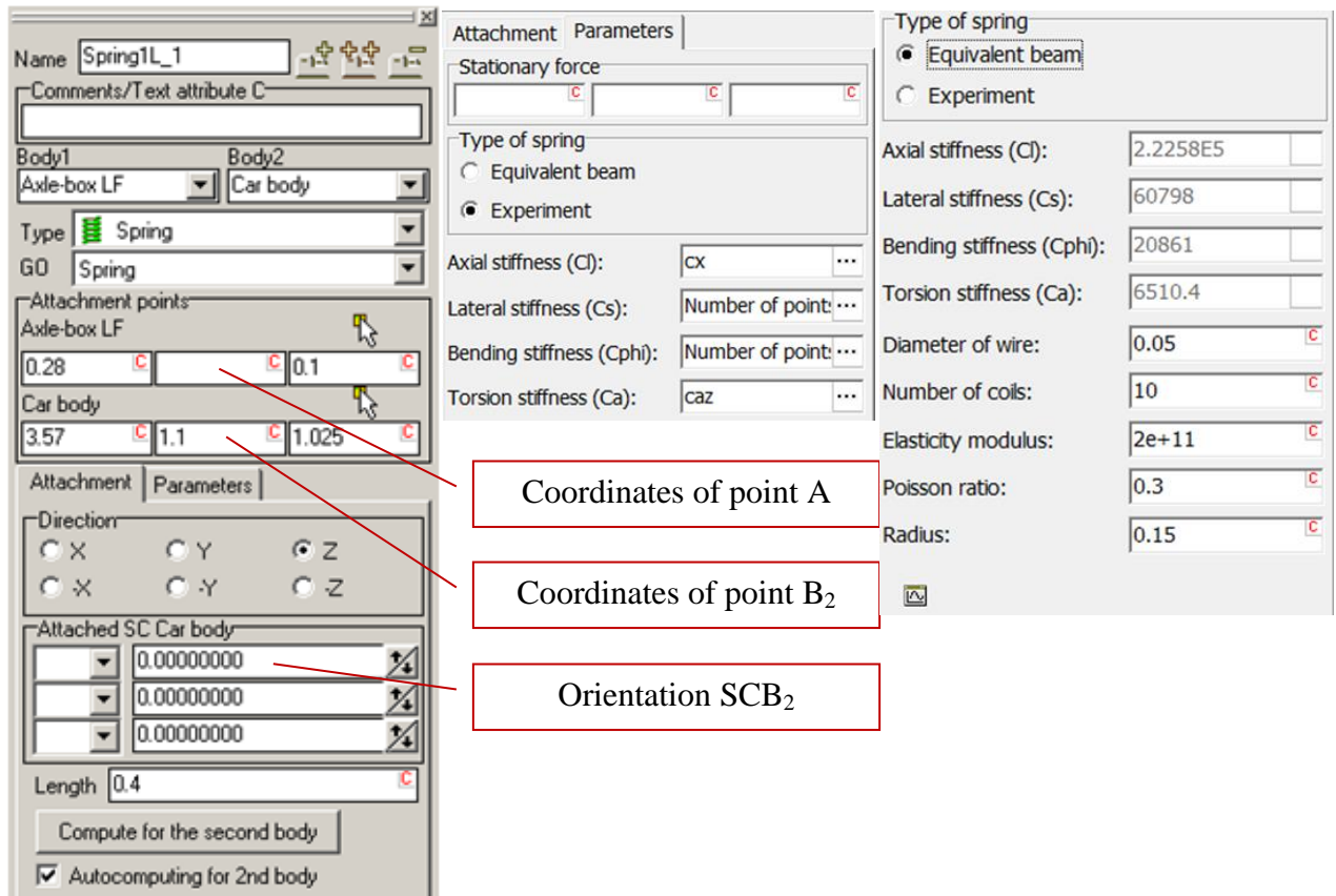
Figure 1.259. Spring parameters
