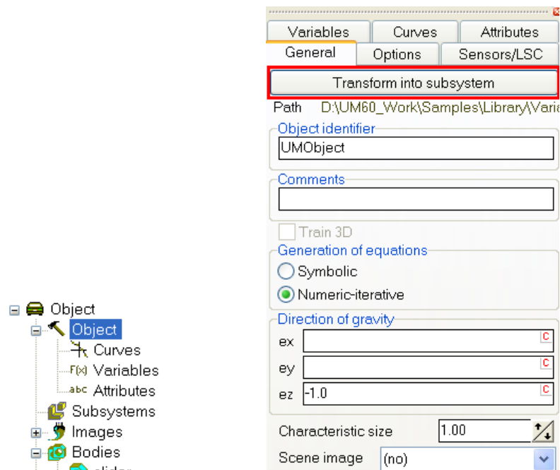
Figure 1.71. Transformation button
