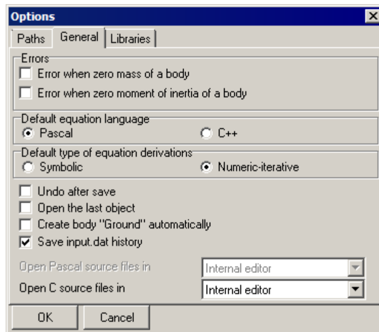
Figure 1.3. General options
