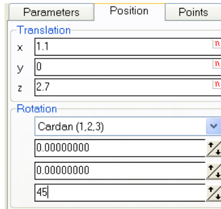
Figure 1.152. Position of body relative to SC0
