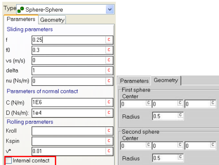
Figure 1.248. Parameters of sphere-sphere contact
