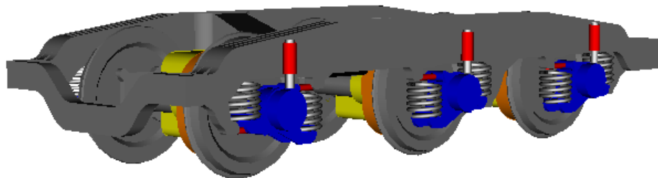
Figure 1.122. Use of GE 'Spring' in the model of a locomotive bogie
