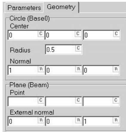
Figure 1.247. Geometric parameters of circle-plane contact
