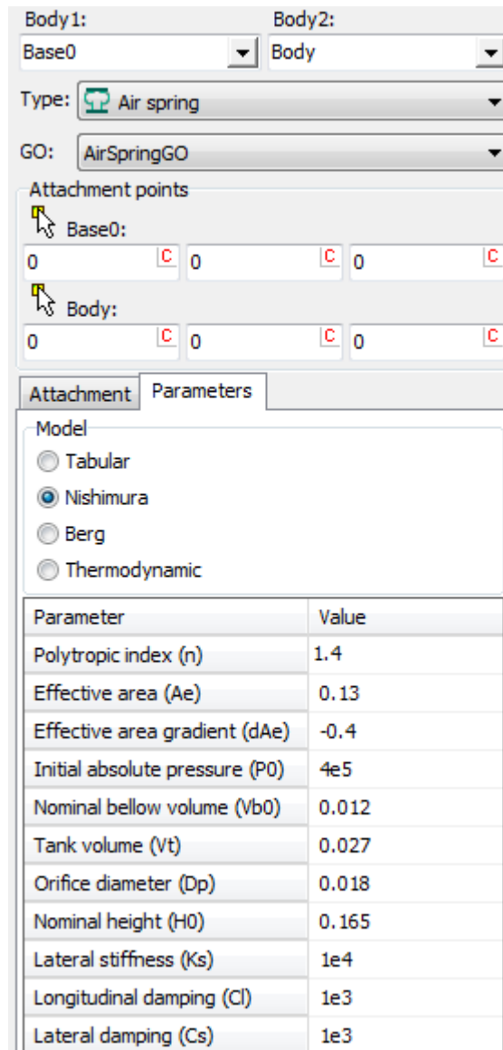
Figure 1.277. Parameters of air spring
