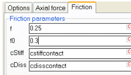
Figure 1.270. Friction force description
