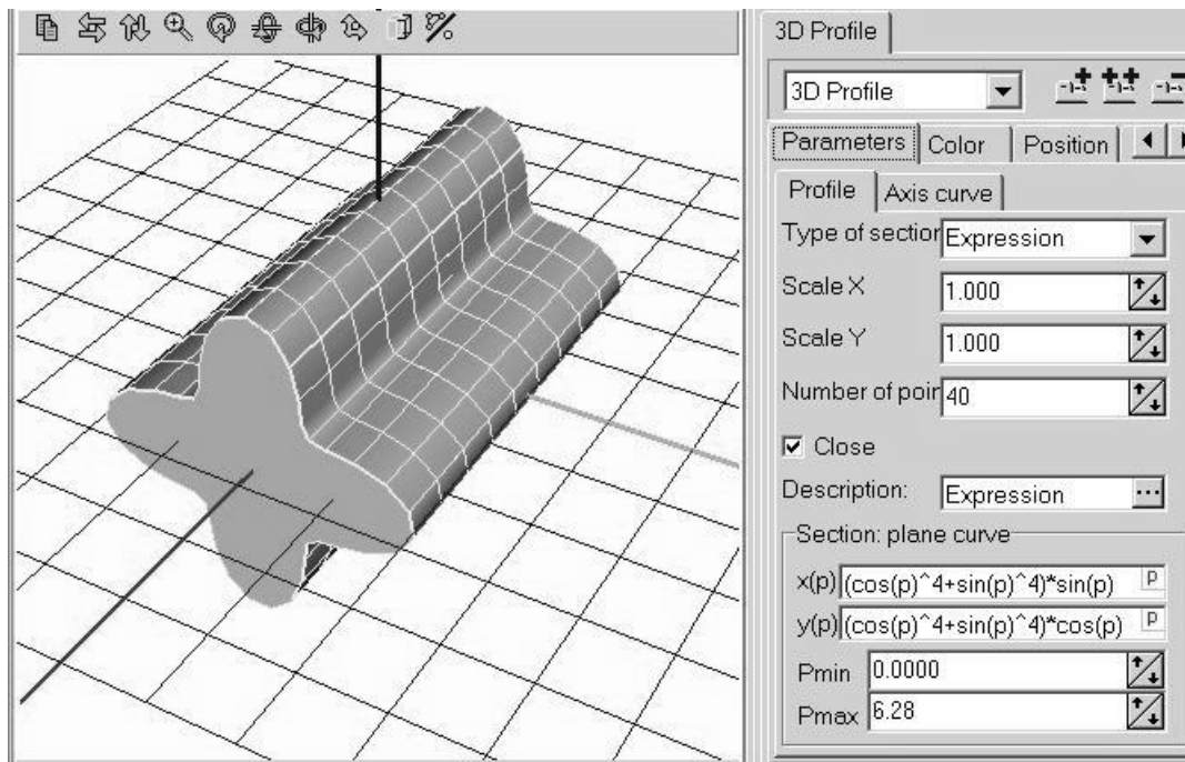
Figure 1.116. Profiled GE: section given by formulas
