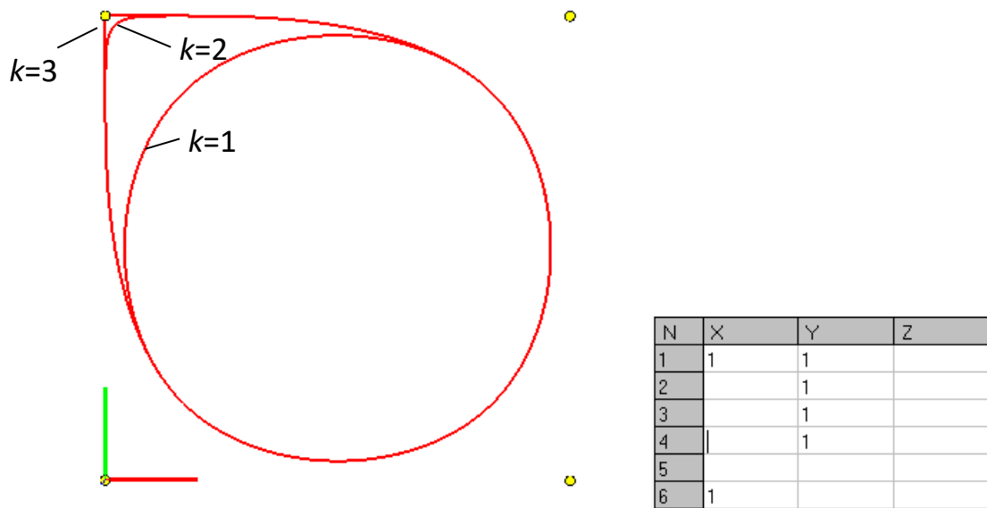
Figure 1.101. Curves with different multiplicity k of the second vertex, m=4 (left). List of vertices in which the second vertex has multiplicity 3
