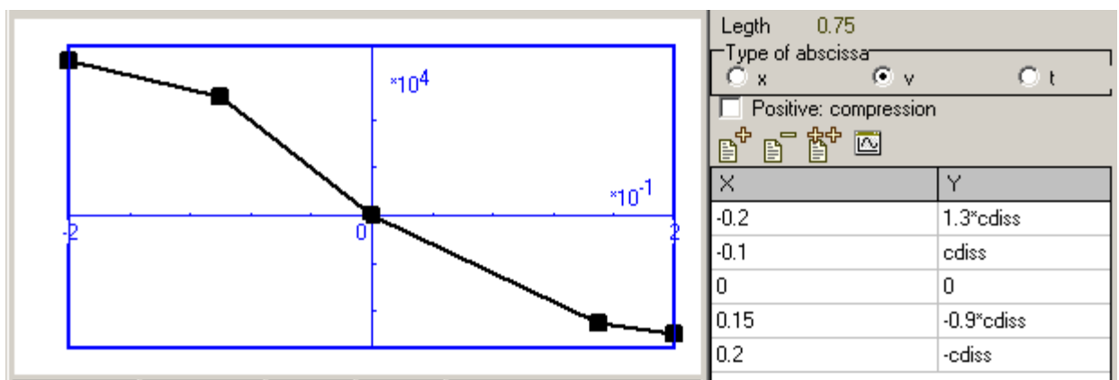
Figure 1.214. Nonlinear damper. The Compression positive option is not checked.
