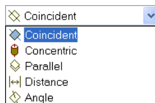
Figure 1.194. Mate types
