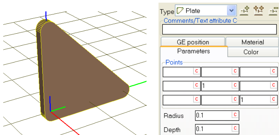
Figure 1.124. Plate parameters
