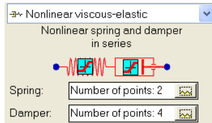
Figure 1.205. Element parameters
