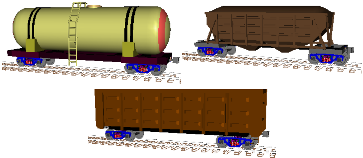
Figure 1.145. Model of a freight car with reassigned images of the car body
