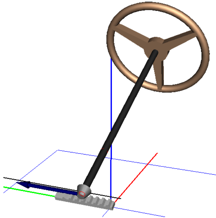
Figure 1.261. Rack and pinion in the car steering system
