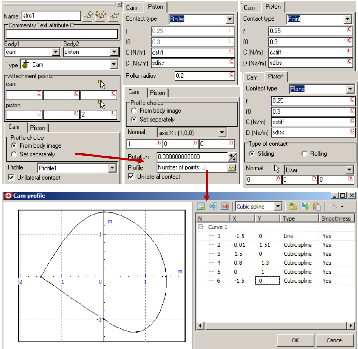
Figure 1.258. Cam parameters
