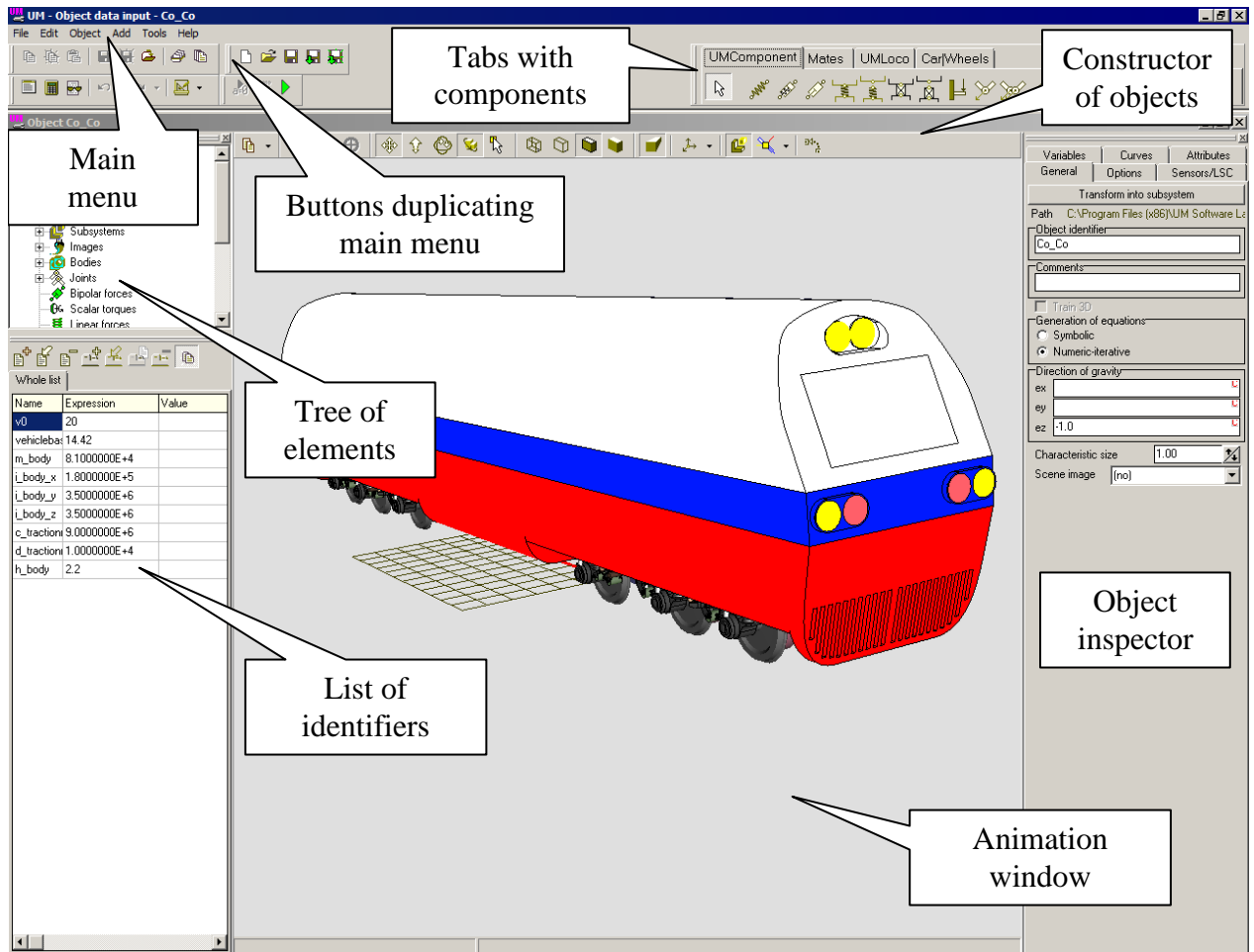
Figure 1.14. Object constructor
