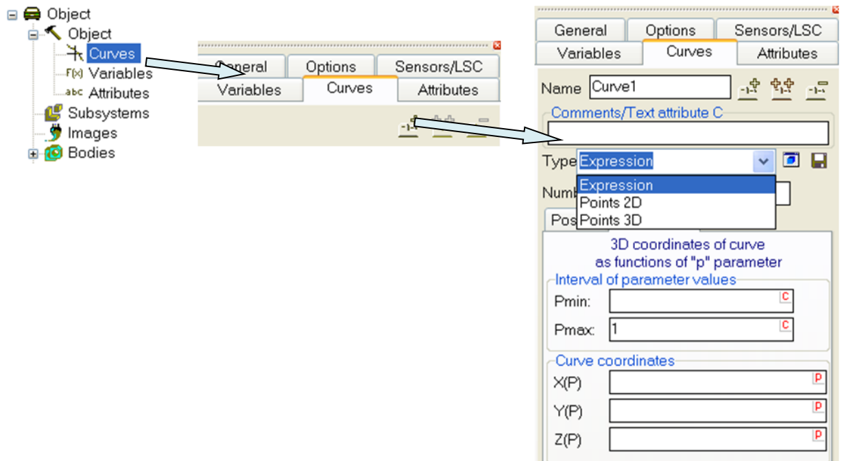
Figure 1.88. New curve
