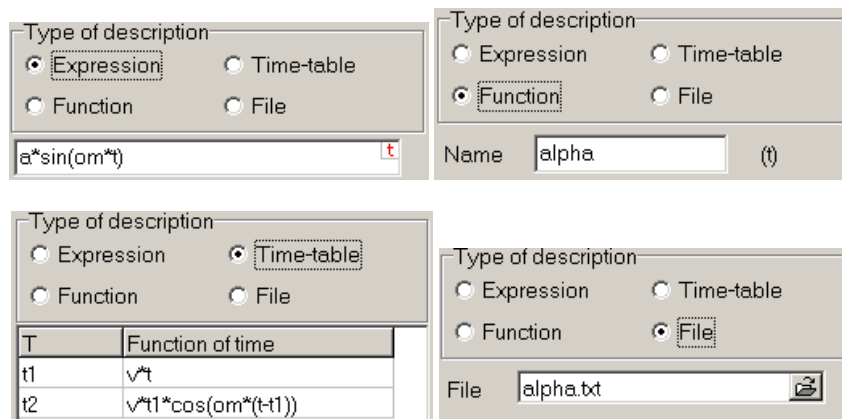
Figure 1.181. Time function
