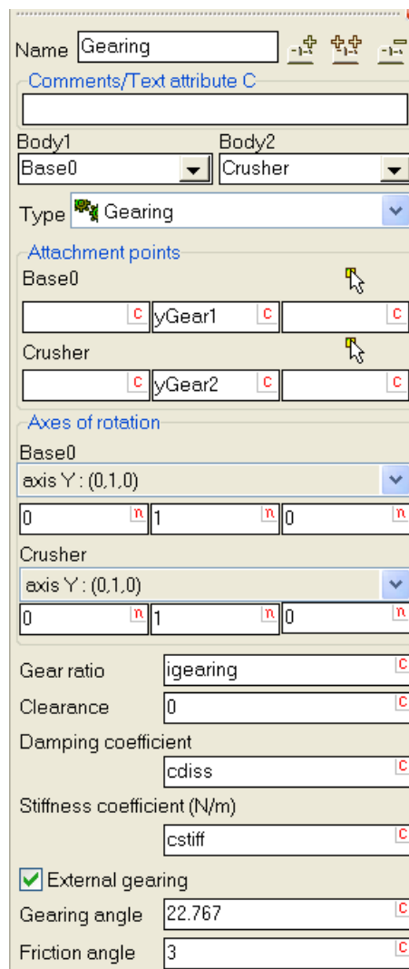
Figure 1.253. Gearing parameters
