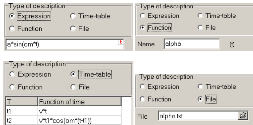
Figure 1.190. Time function
