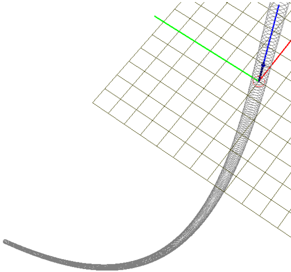
Figure 1.244. Cylinder image
