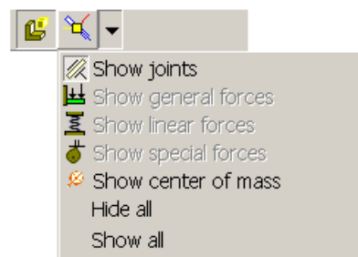
Figure 1.16. Visualization commands
