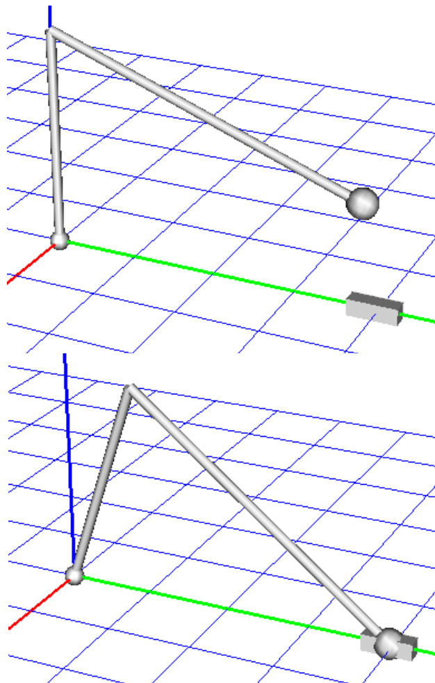
Figure 1.173. Crank-rod mechanism with open and closed cut joint
