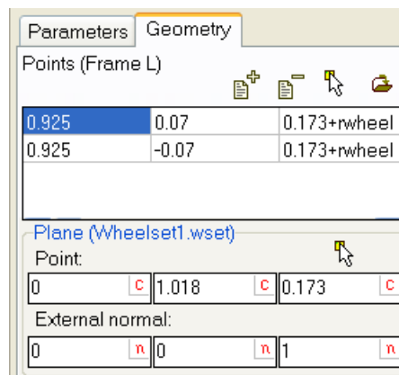
Figure 1.235. Geometry of points-plane contact
