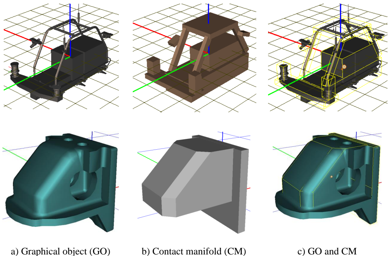
Figure 1.161. Graphical object and contact manifold for a body of wheeled robot
