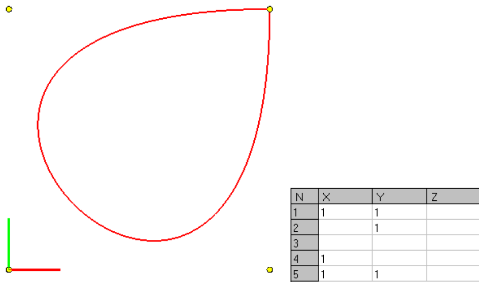
Figure 1.99. Closed unperiodic B-spline, m=4
