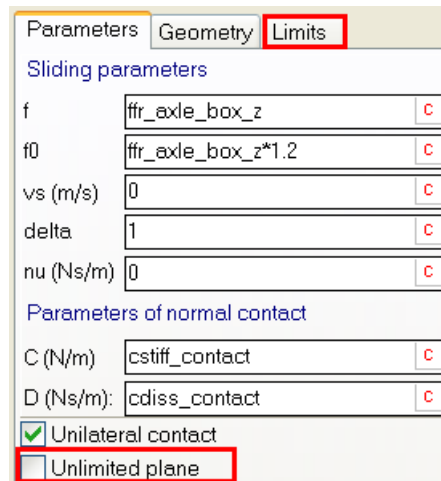
Figure 1.238. Mode of limited contact plane
