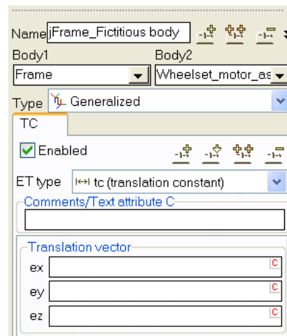
Figure 1.80. Joint rigidly connecting a frame with a fictitious body
