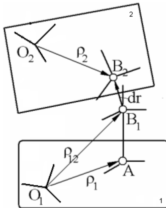
Figure 1.283. Systems of coordinates related to linear force elements
