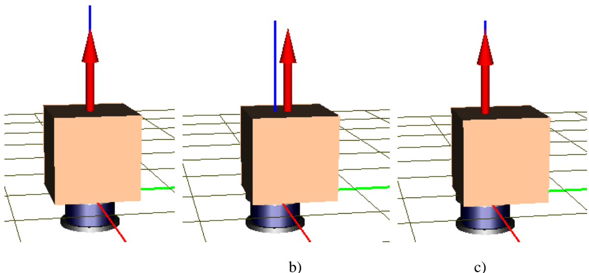
Figure 1.274. Position of the normal force by shift of the second body. The contact point belongs to the first body (b) or the first body (c)
