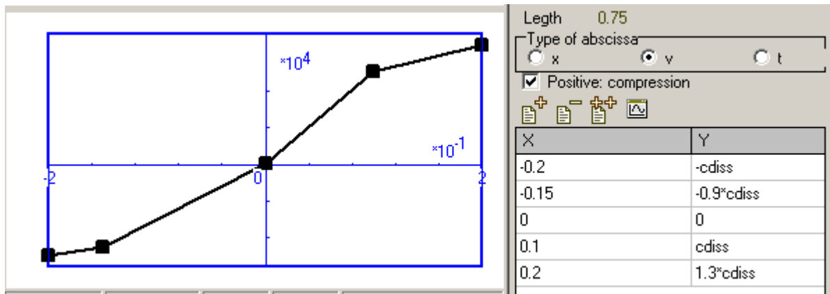
Figure 1.215. Nonlinear damper. The Compression positive option is checked.
