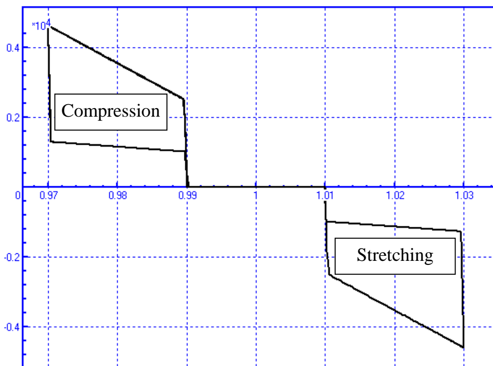
Figure 1.220. Example of hysteretic element with symmetric operation relative to length 1 m
