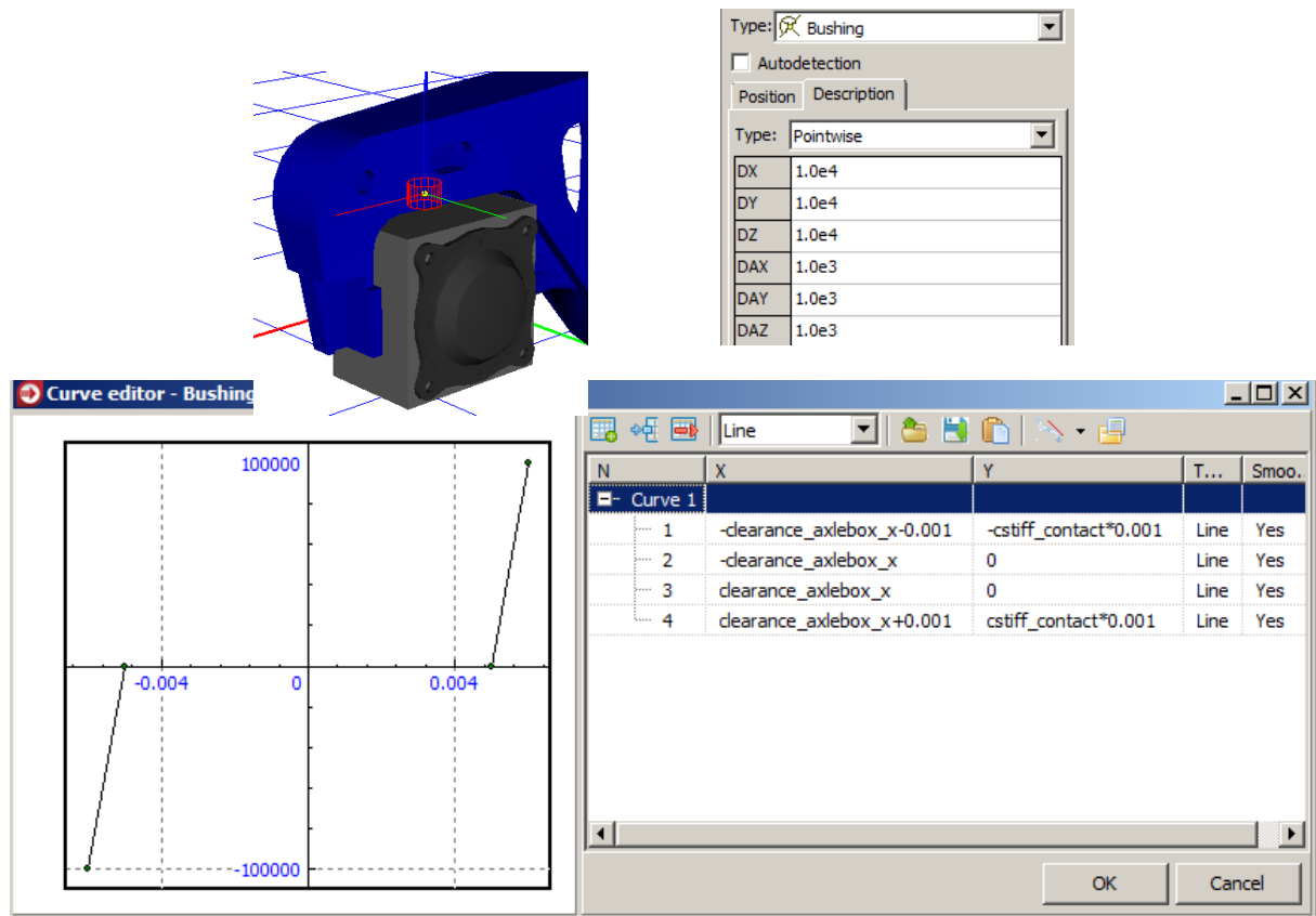
Figure 1.264. Example of a pointwise bushing, which is used for modeling support and gaps between a side frame and an axle-box in the model of a three-piece bogie of a freight car
