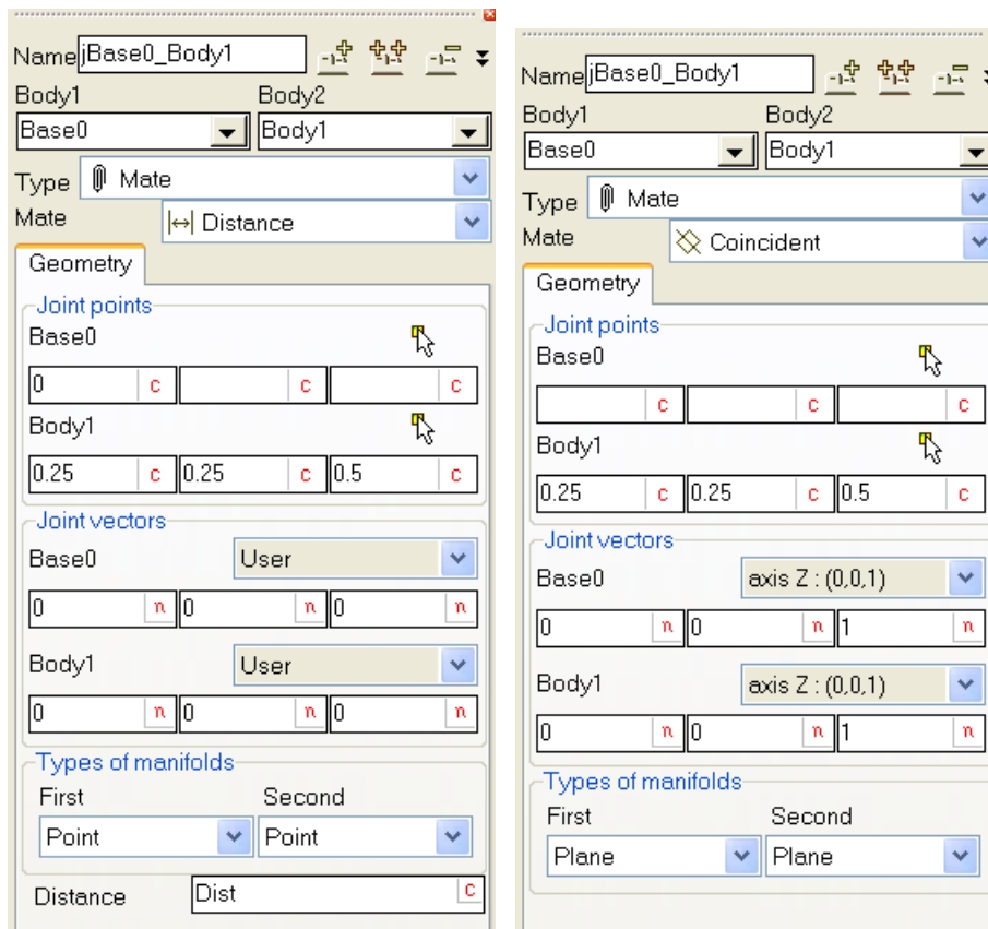
Figure 1.193. Examples of mates
