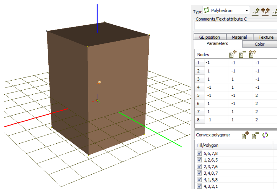
Figure 1.147. Correct enumeration of vertices of a polyhedron when automatic computing inertia parameters
