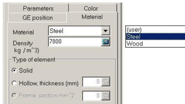
Figure 1.133. Inertia parameters of GE material
