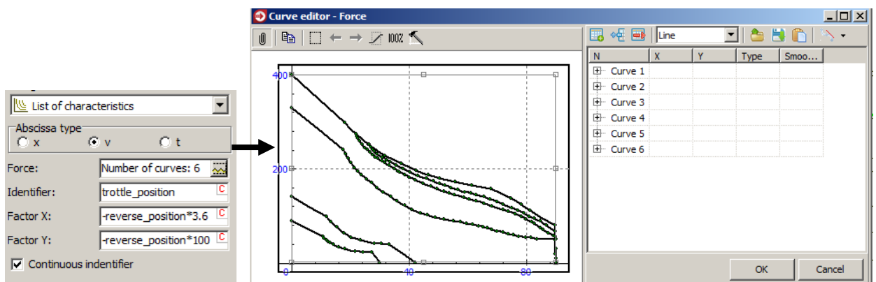
Figure 1.217. Example of a traction force model as a list of characteristics
