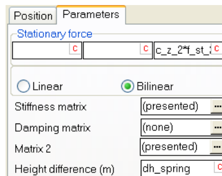
Figure 1.232. Parameters of bilinear force element
