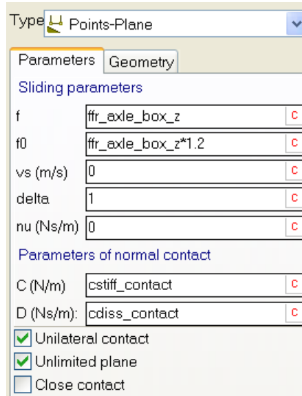
Figure 1.234. Parameters of 'points-plane' contact force
