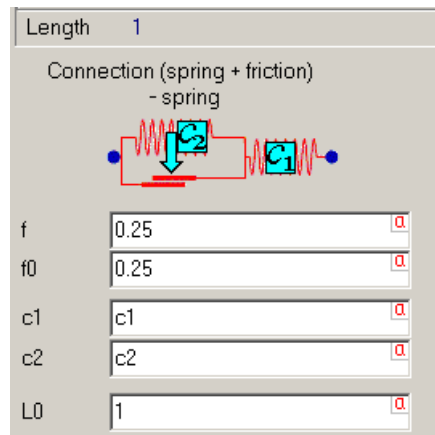
Figure 1.203. Parameters of elastic-friction element 2
