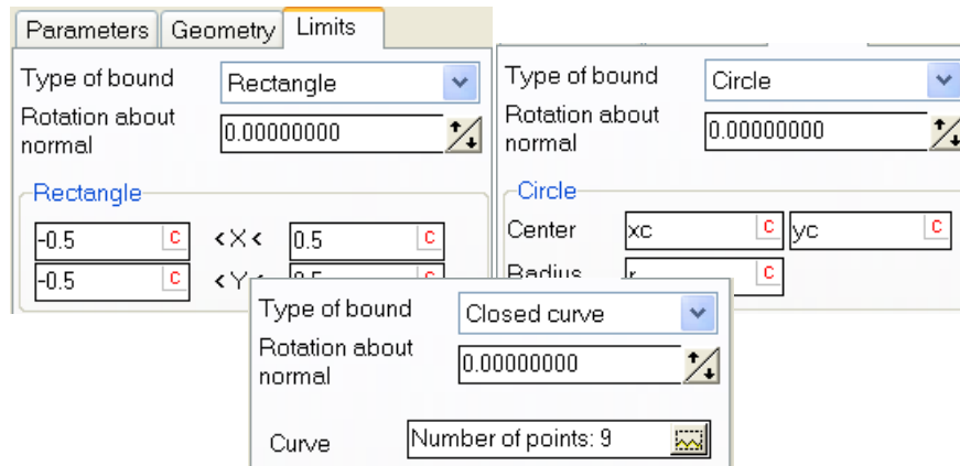
Figure 1.239. Different bounds of the contact area
