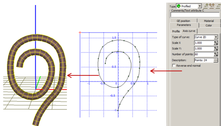
Figure 1.117. Profiled GE: a 2D axis curve given by points
