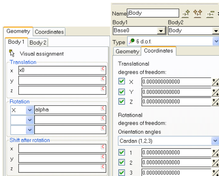
Figure 1.182. Description of 6 d.o.f. joint
