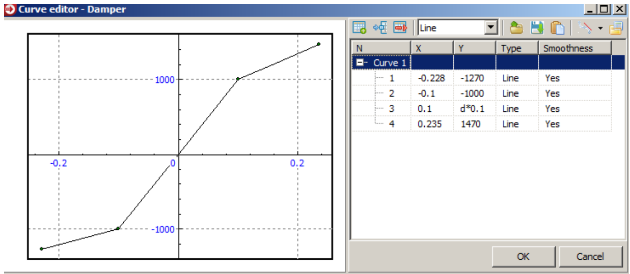
Figure 1.207. Parameterized model of nonlinear damper
