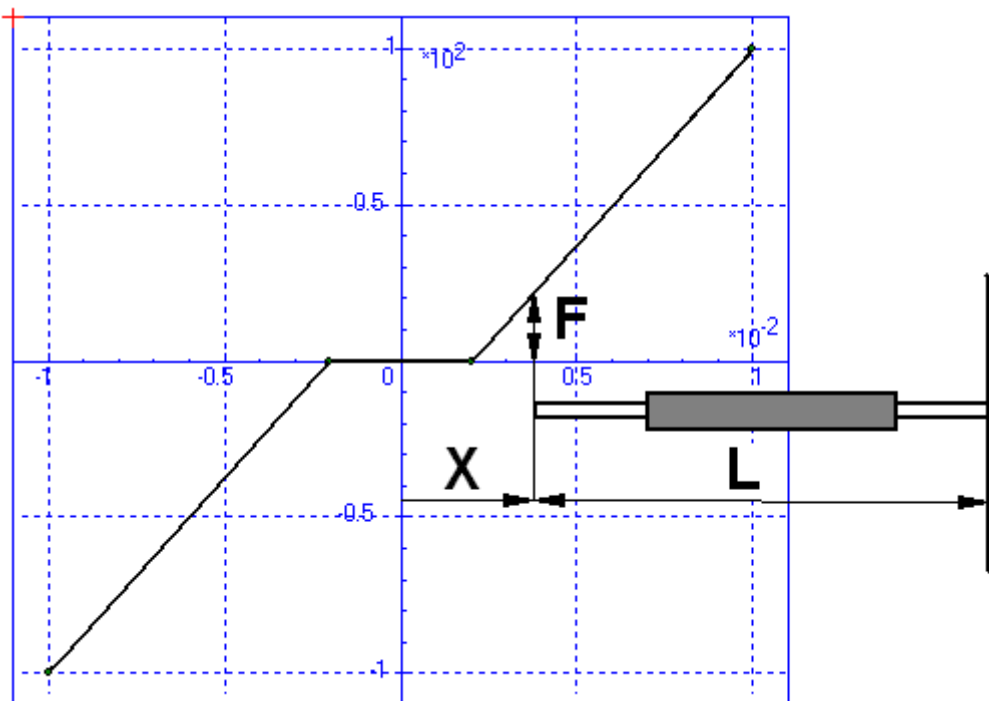
Figure 1.211. To the notion of abscissa matching. The Compression positive option is checked.
