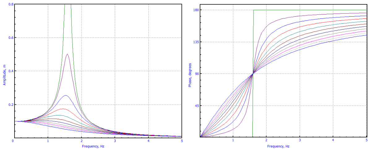
Figure 1.191. Amplitude and phase of oscillations versus frequency for 1 DOF oscillator
