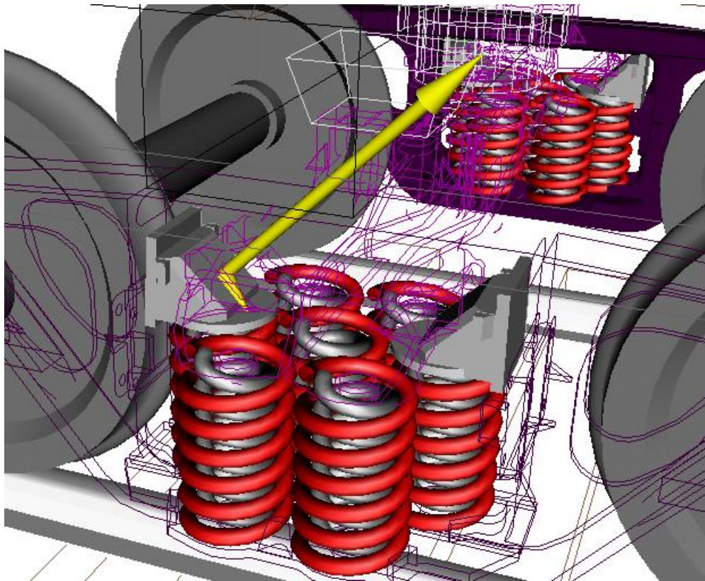
Figure 1.30. Principal vectors of normal and friction forces acting on the bolster from the wedge
