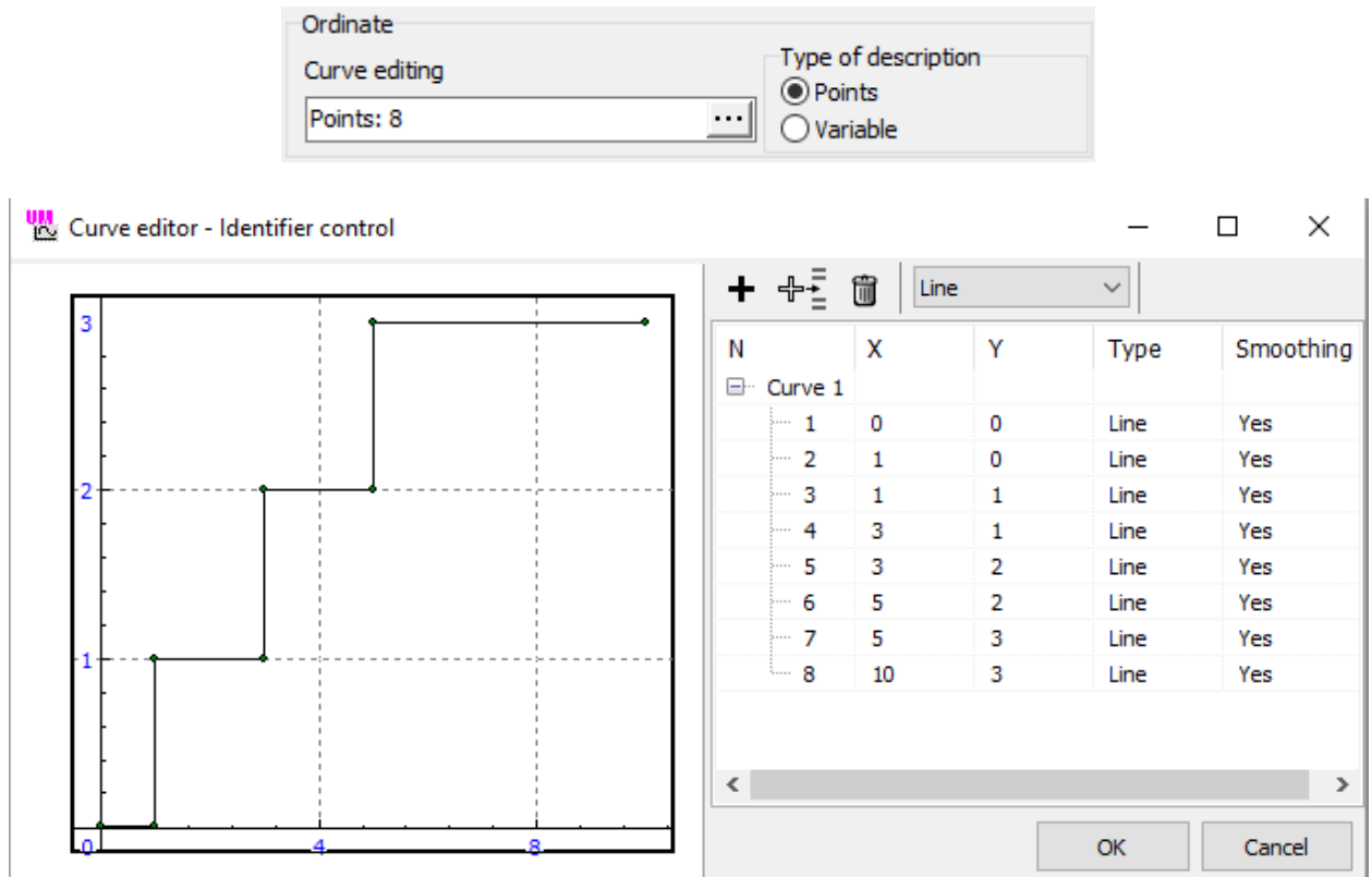
Figure 1.106. Example of pointwise function
