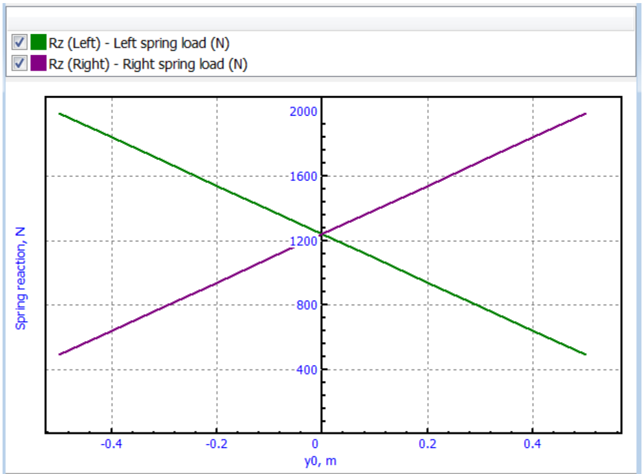
Figure 1.184. Static spring forces versus coordinate of load application
