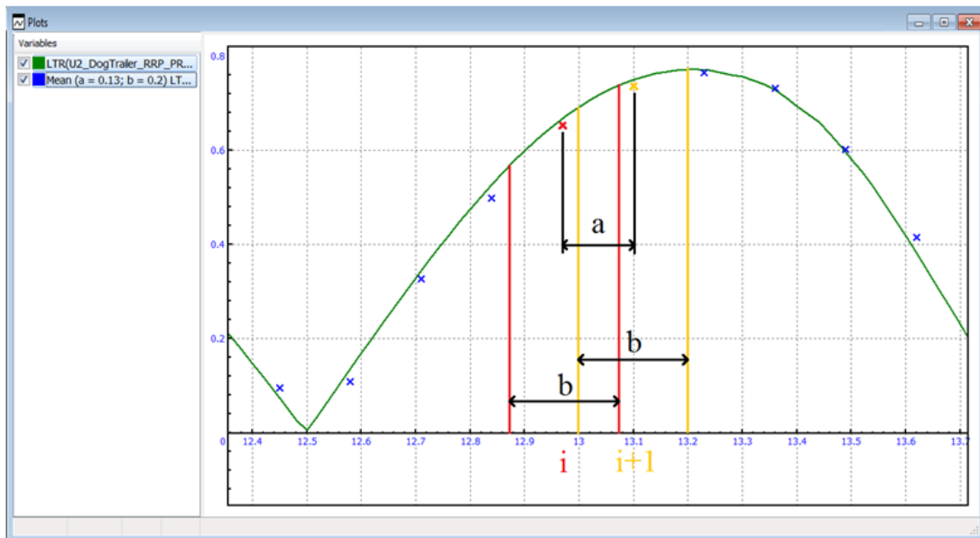
Figure 1.59. Example of interval statistic (functional – mean value, a = 0.13 m, b = 0.2 m)
