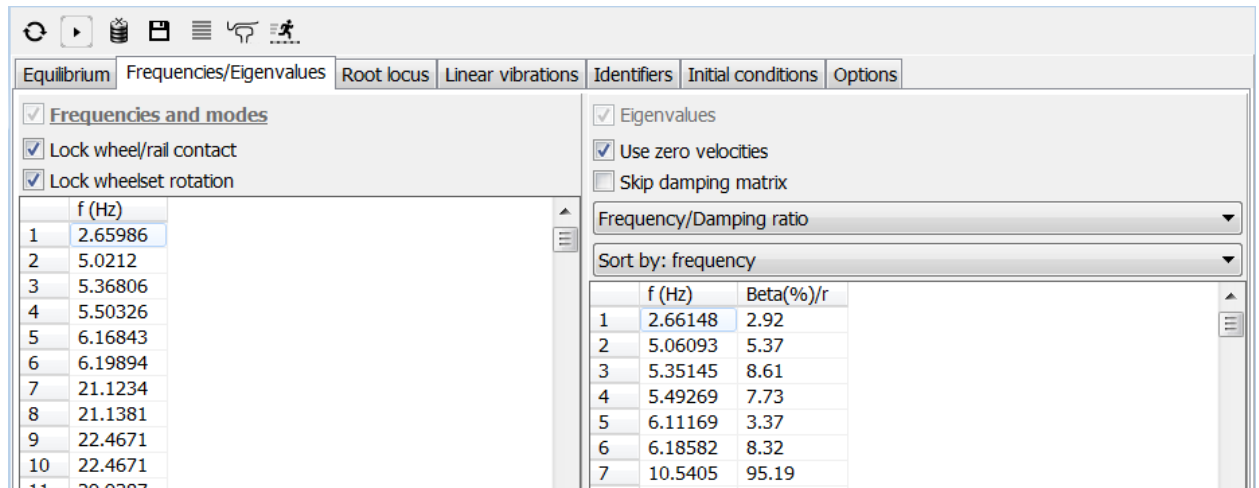
Figure 1.143. Natural frequencies and eigenvalues
