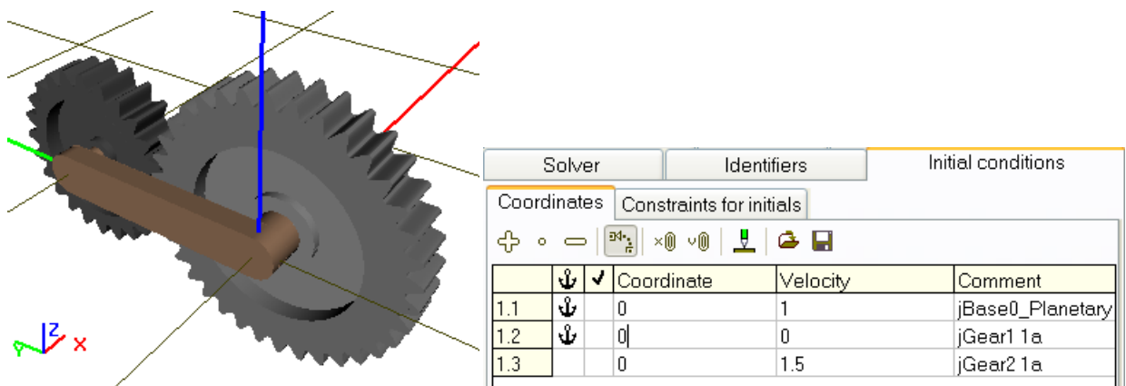
Figure 1.111. Planetary train model and table of coordinates
