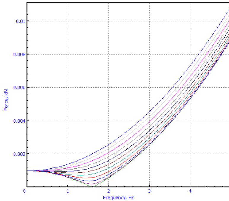
Figure 1.192. Amplitude of excitation force for kinematic excitations of oscillator
