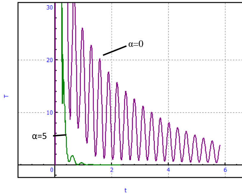
Figure 1.130. Kinetic energy time history by computation of equilibrium
