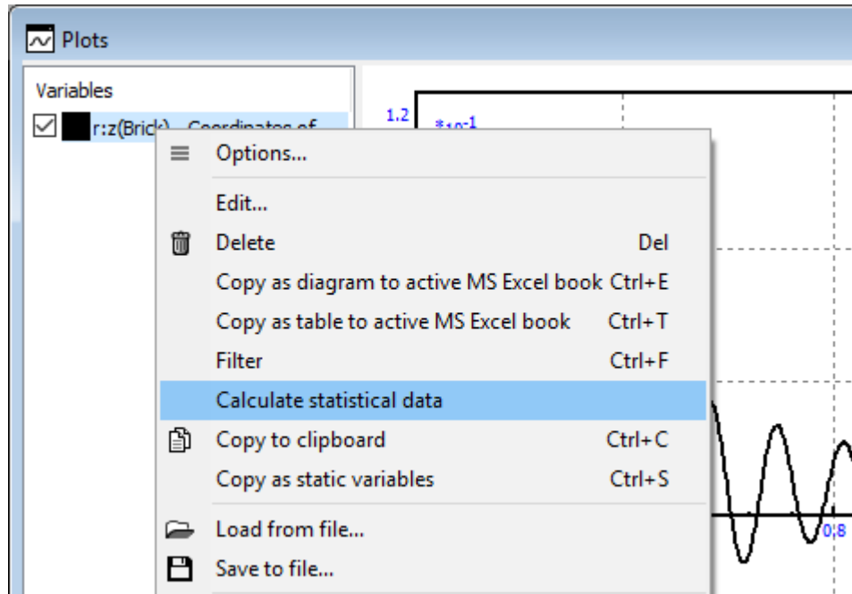
Figure 1.56. Statistic command
