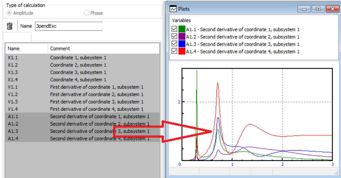
Figure 1.167. Amplitudes of acceleration vibrations vs. frequency
