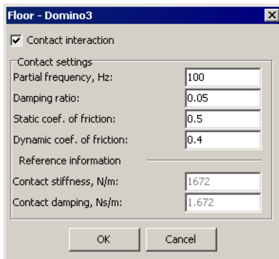
Figure 1.118. Parameters of contact interaction between two bodies
