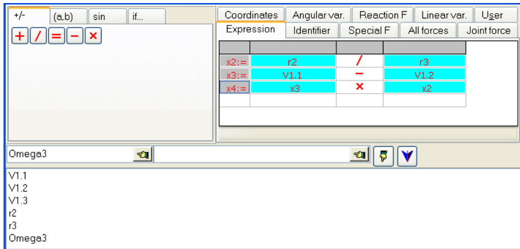
Figure 1.113. Expressions for computation of angular velocity of the planet gear
