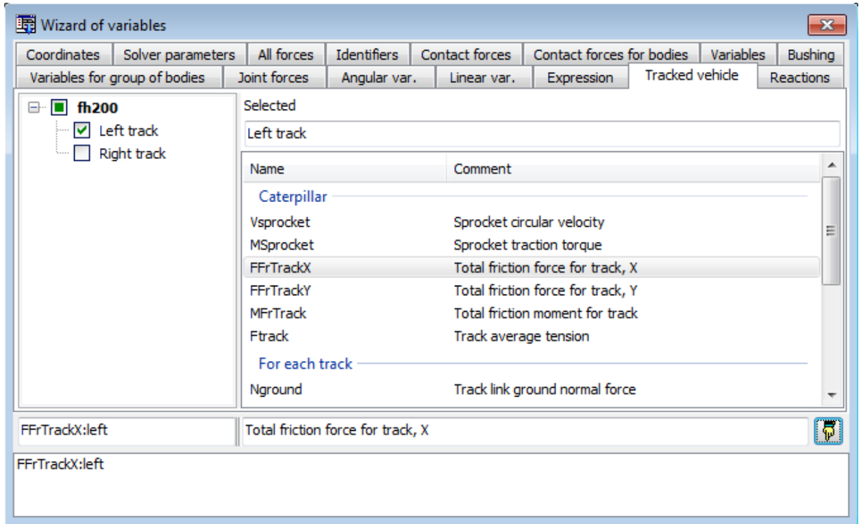
Figure 1.39. Special variables for a tracked vehicle
