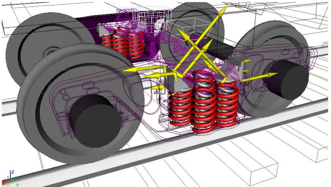
Figure 1.28. Vectors of contact forces
