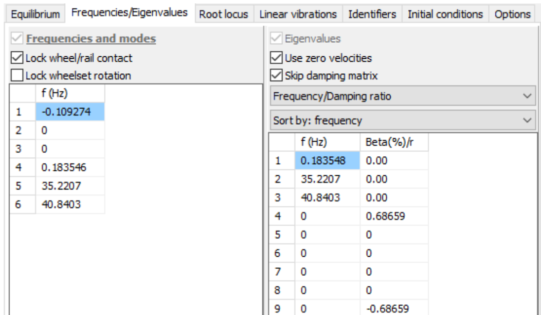
Figure 1.188. Computed natural frequencies and EVs for a wheelset on smooth rails
