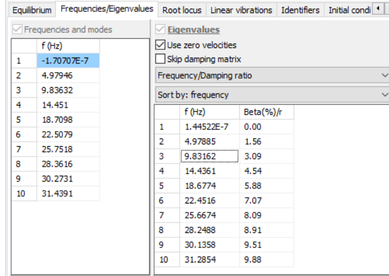
Figure 1.186. Computed frequencies and EVs of the chain
