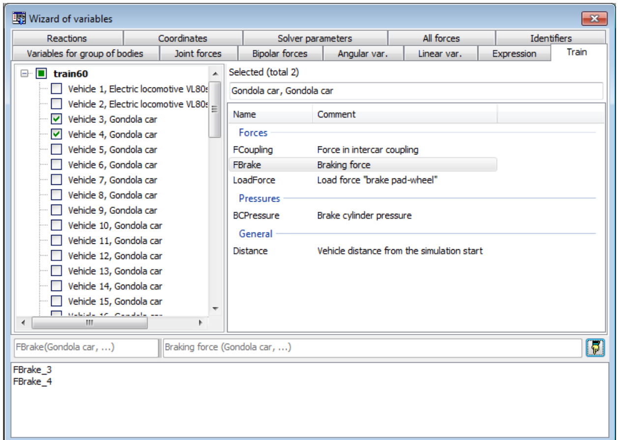
Figure 1.40. Special variables for a train
