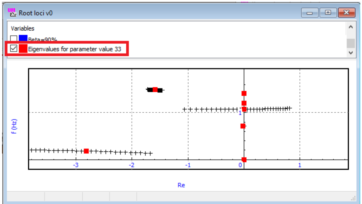
Figure 1.160. Dependence of stability for identifier v0
