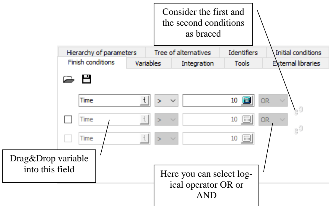
Figure 1.12. User-defined finish conditions
