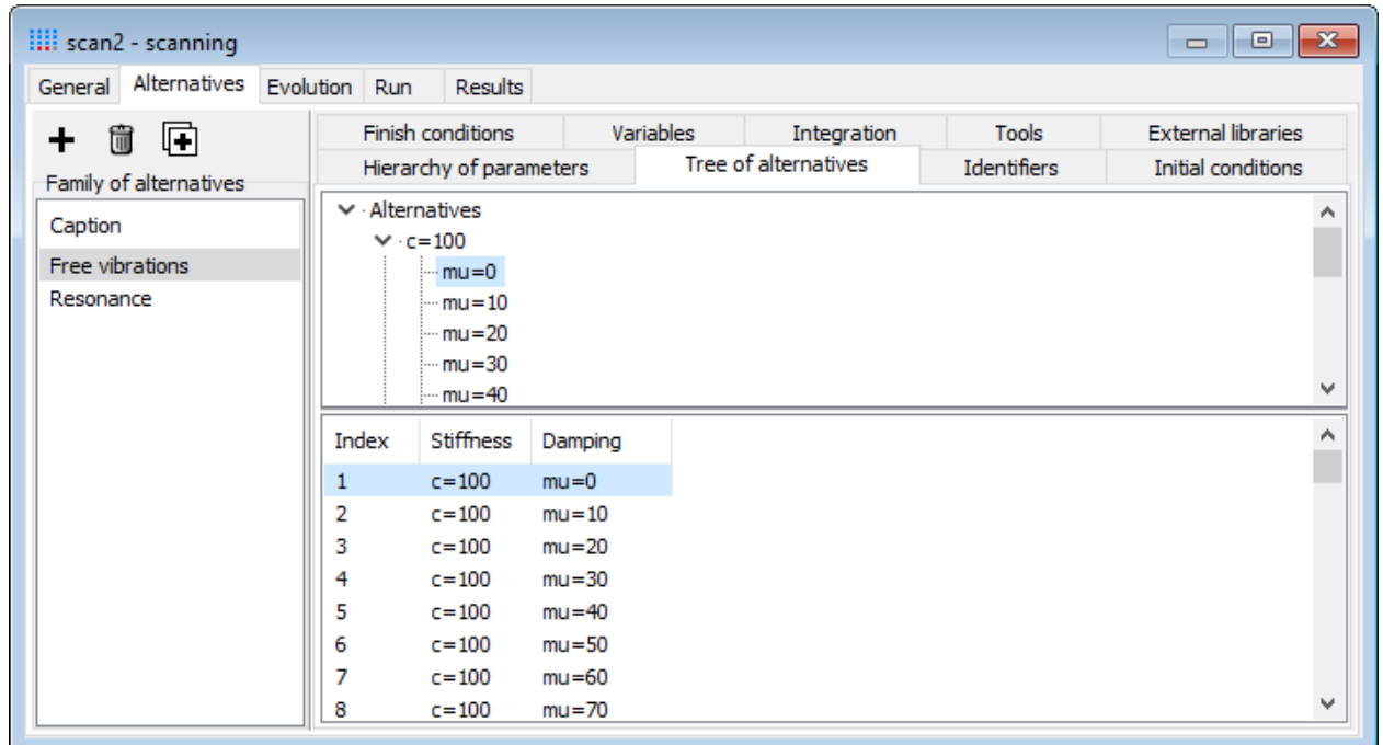
Figure 1.10. Tree of alternatives
