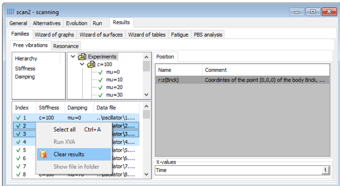
Figure 1.6. Deleting simulation results for some experiments
