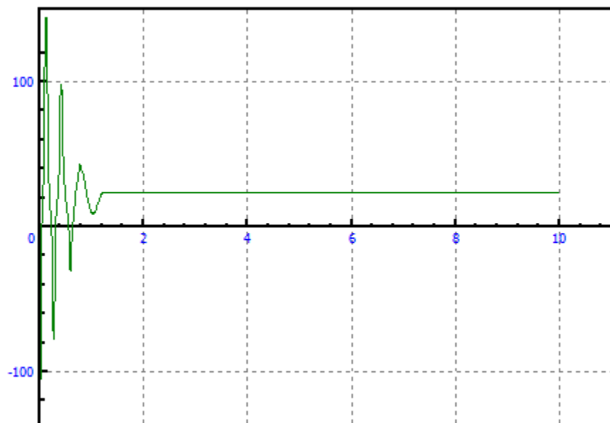
Figure 1.46 Friction force
