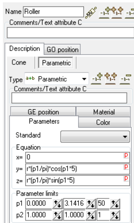
Figure 1.30. Definition of parametric graphic image
