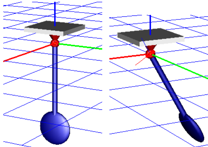
Figure 1.38. Pendulum with horizontal and inclined rotation axis
