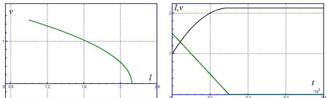
Figure 1.4. Box velocity versus lateral position (left); box velocity and lateral position versus time (right)
