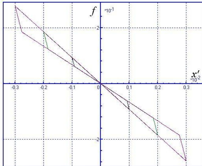
Figure 1.9. Force versus displacement
