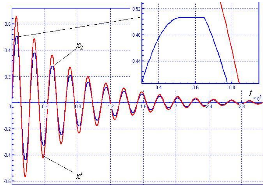
Figure 1.13. Full element deflection x' = x - L_0 and spring in parallel friction deflection x_2 versus time
