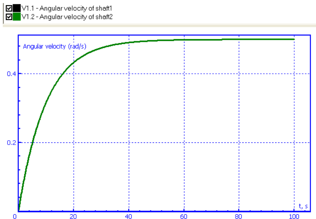
Figure 1.16. Shaft angular velocities vs time
