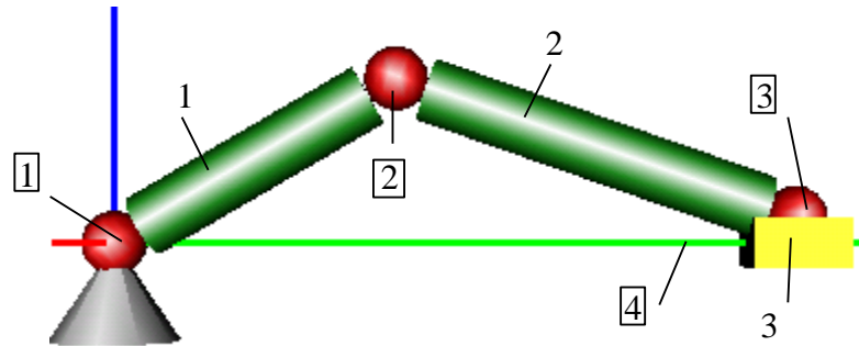
Figure 1.34. Slider-crank mechanism
