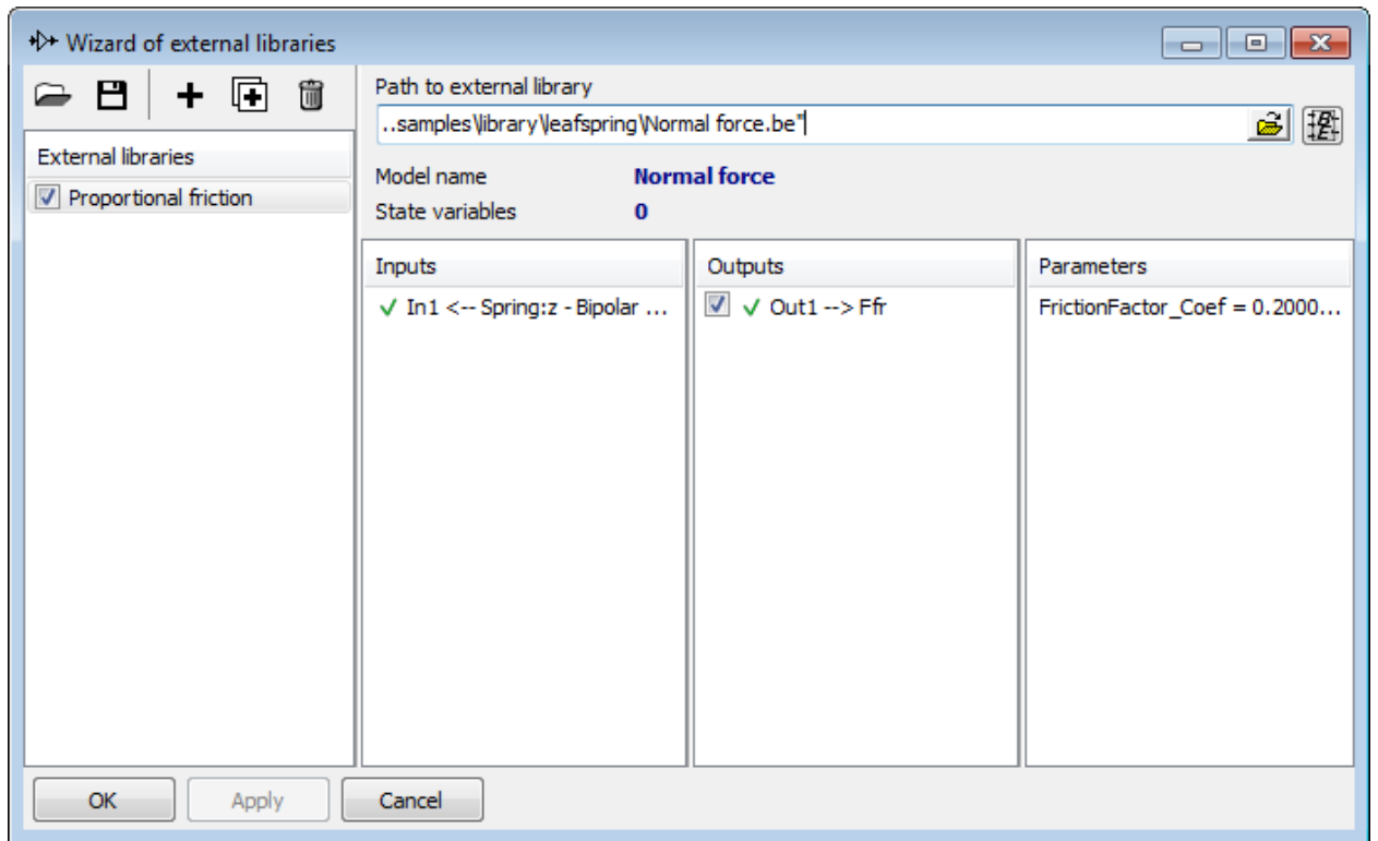
Figure 1.45 Wizard of external libraries
