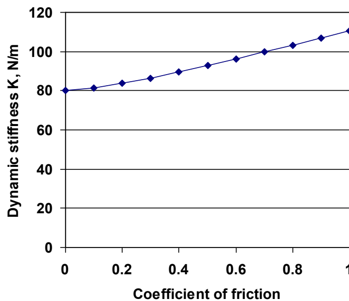
Figure 1.10. Dynamic stiffness versus coefficient of friction
