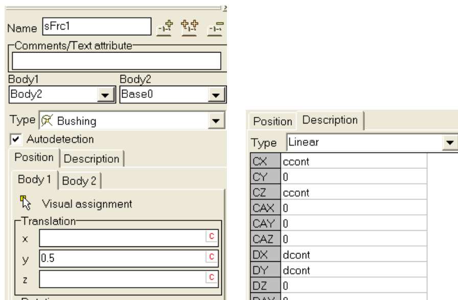
Figure 1.15. Force element of ‘bushing’ type
