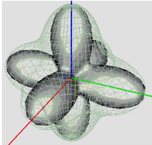
Figure 1.37. Molecule
