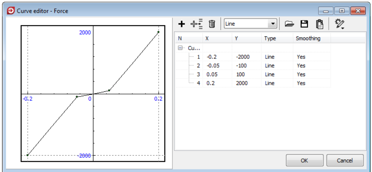
Figure 1.43 Axial force
