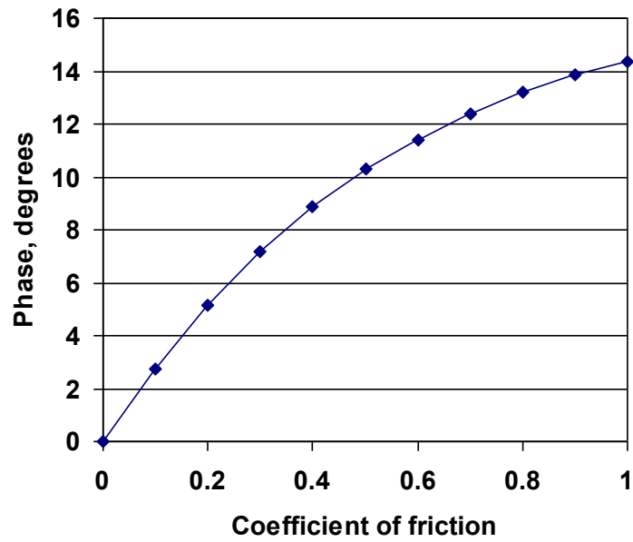
Figure 1.11. Phase versus coefficient of friction
