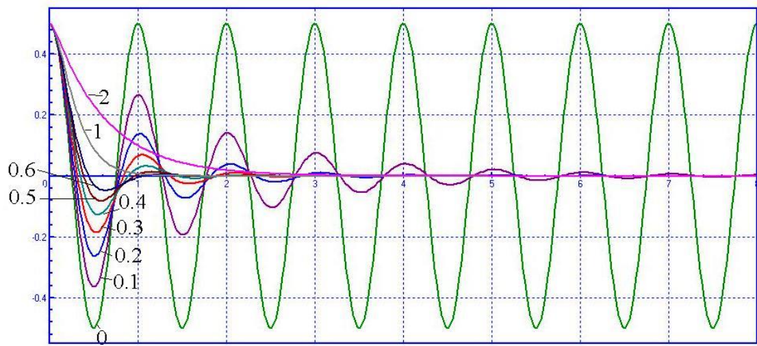
Figure 1.2. Damped oscillations for different values of damping ratio
