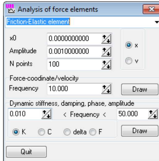
Figure 1.8. Window for analysis of forces in frequency domain
