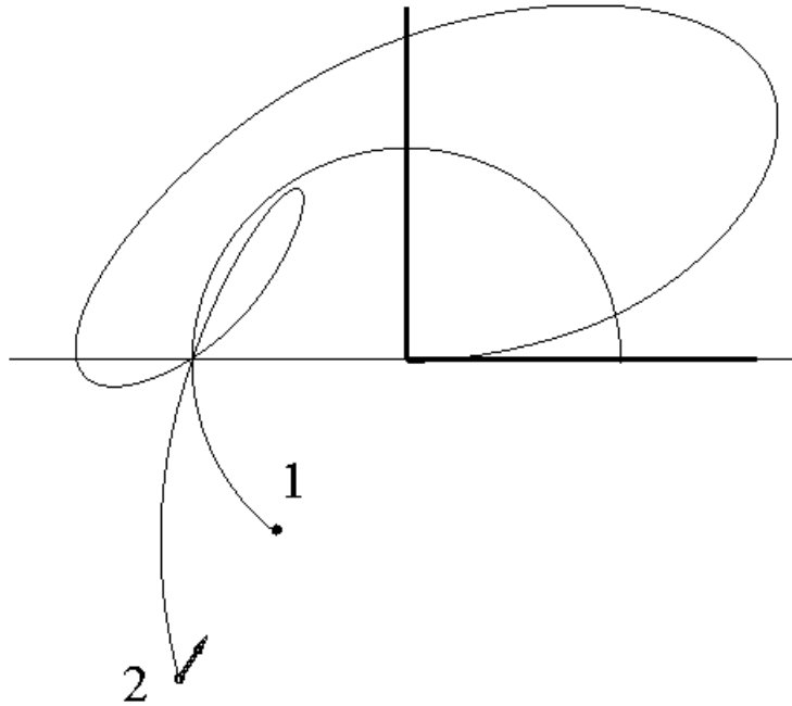
Figure 1.35. Pursuit game
