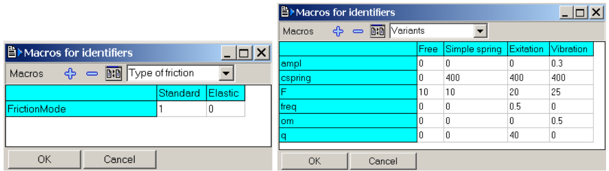
Figure 1.3. Macro-commands
