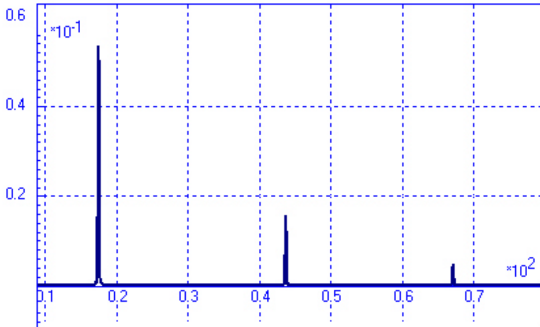
Figure 1.26. Power spectral density of oscillation of body 3
