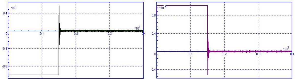
Figure 1.5. Friction force versus time (left); elastic deflection versus time (right)
