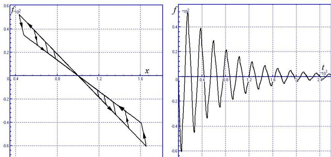
Figure 1.12. Force versus element length and time
