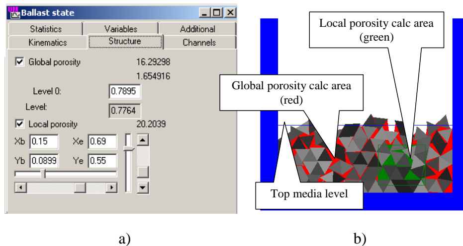
Figure 1.10. Information about structure of a ballast: a) Structure tab; b) graphic presentation of some parameters.
