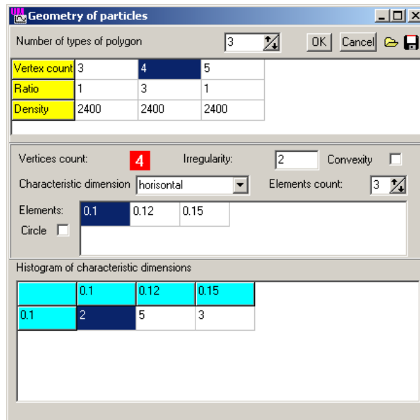
Figure 1.8. A dialog is Geometry of particles
