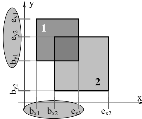
Figure 1.3. Illustration to the method of the constrained linear lists.
