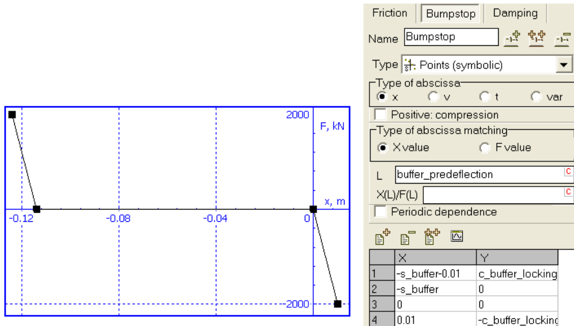
Figure 1.34. Limitation in the draft gear travel
