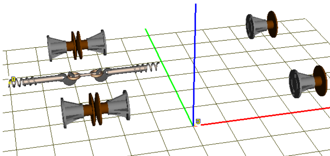
Figure 1.27. Model of buffer coupling system, UM object Buffer_Ext_R
