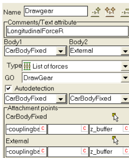
Figure 1.36. Draw gear element
