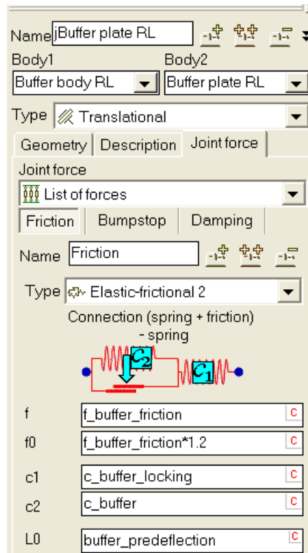
Figure 1.32. Draft gear friction model
