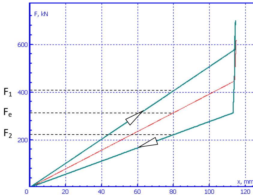
Figure 1.33. Draft gear hysteresis
