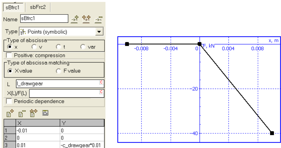
Figure 1.37. External element: draw gear working on stretching. Elastic component
