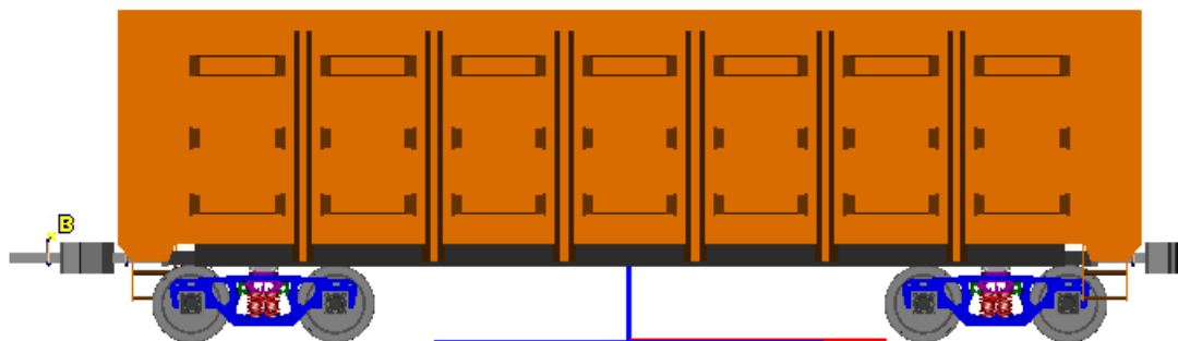
Figure 1.9. Model simple_18_100_AC_ExtR of a freight vehicle with automatic coupler system according to the model AC_Standard_EXT_R
