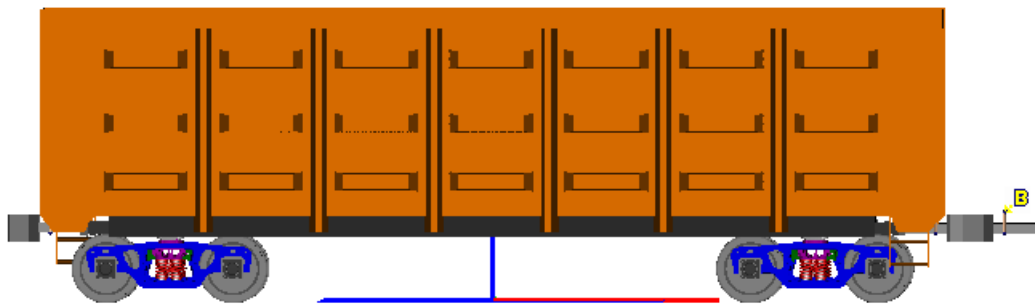
Figure 1.8. Model simple_18_100_AC_ExtF of a freight vehicle with automatic coupler system according to the model AC_Standard_EXT_F
