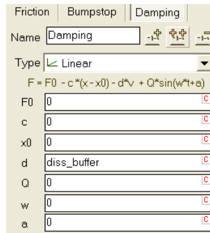
Figure 1.35. Linear damping
