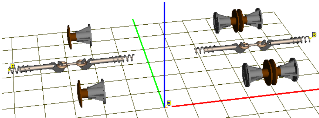
Figure 1.26. Model of buffer coupling system, UM object Buffer_Ext_F
