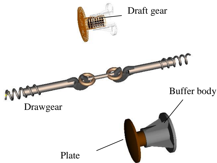
Figure 1.31. Structure of model
