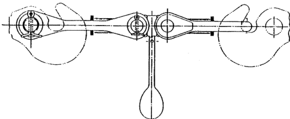
Figure 1.24. Drawgear
