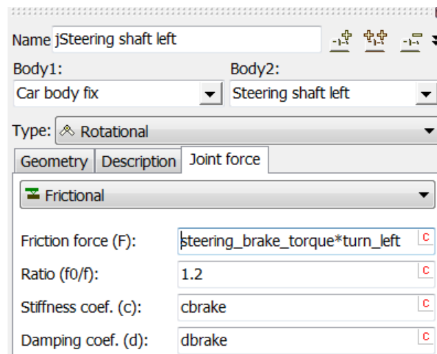
Figure 1.136. Steering brake torque
