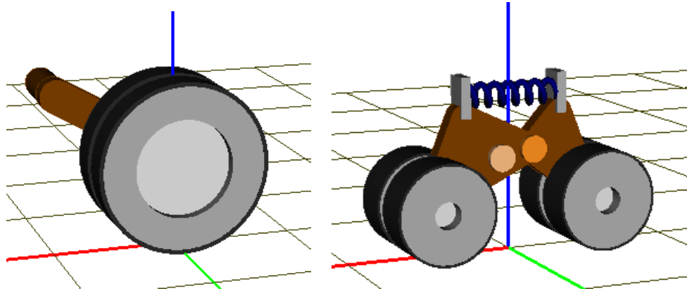
Figure 1.5. Examples of subsystems describing elements of suspension. Torsion bar and joint bogie suspensions
