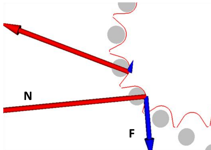
Figure 1.140. Pin-sprocket forces
