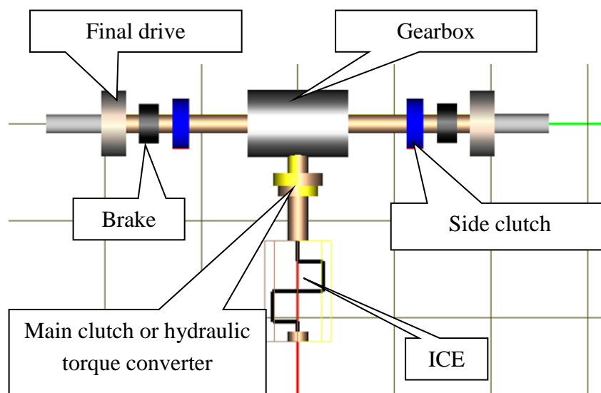
Figure 1.108. Transmission with Clutch-Brake steering mechanism
