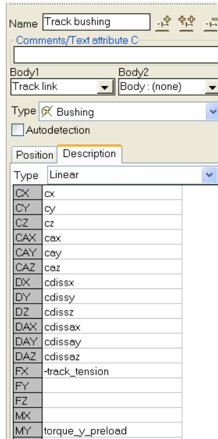
Figure 1.64. Parameters of bushing
