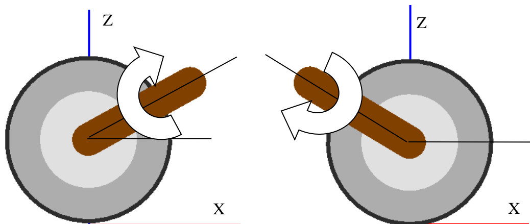
Figure 1.19. Direction of positive rotation in joint
