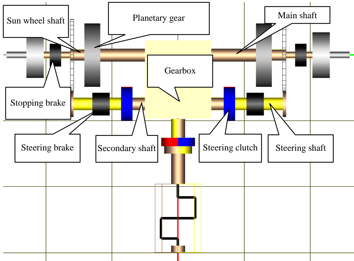
Figure 1.135. Modified double differential steering system
