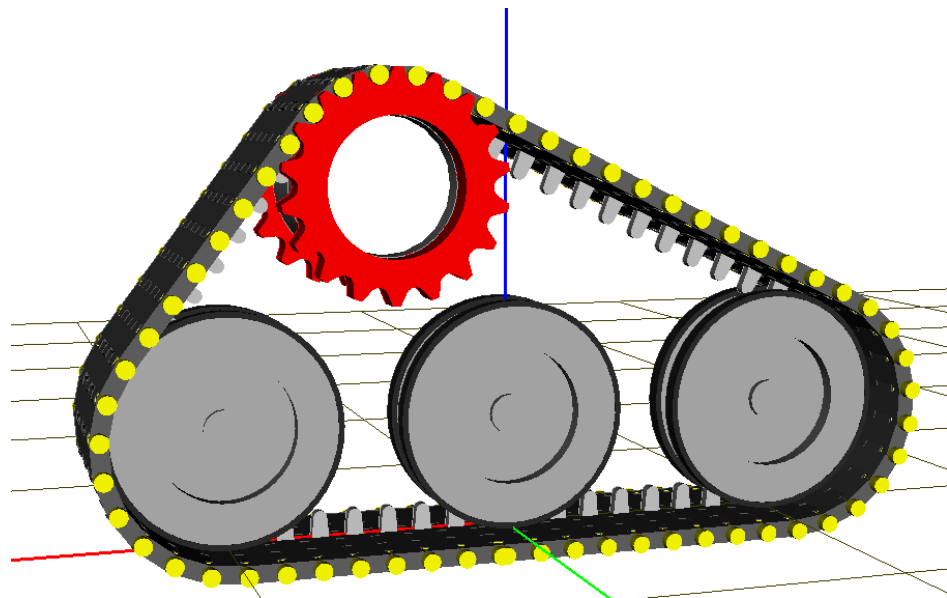
Figure 1.82. Example of a track without an idler
