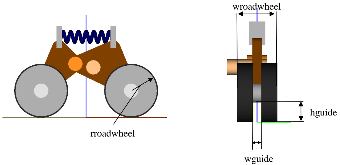
Figure 1.9. Standard geometrical identifiers
