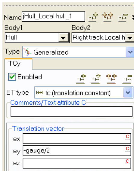
Figure 1.104. Joint rigidly connecting the local hull of the right track with the hull of TV
