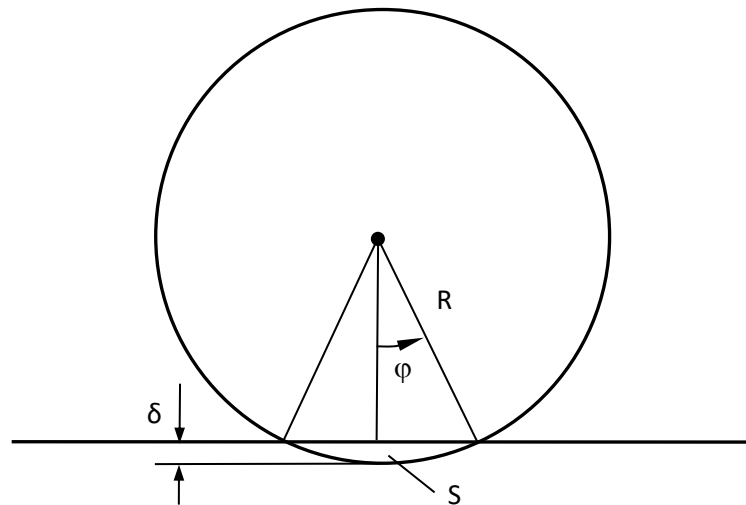
Figure 1.145. Penetration of a wheel into a plane
