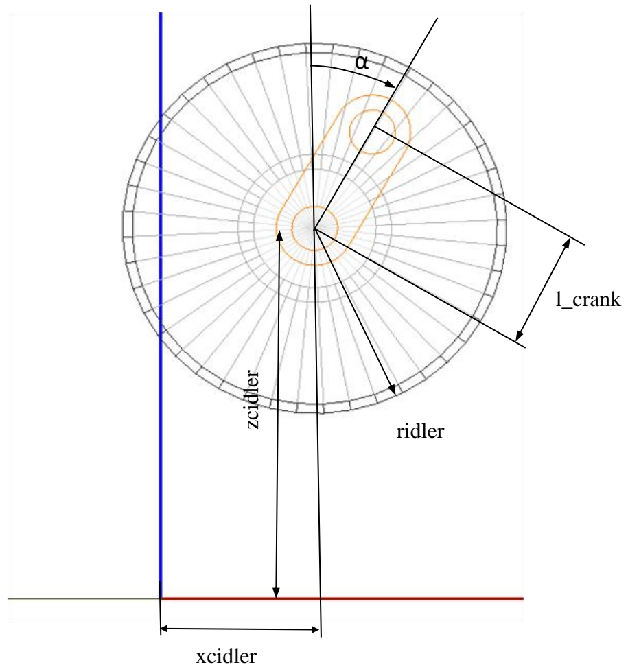
Figure 1.36. Geometric parameters of the model
