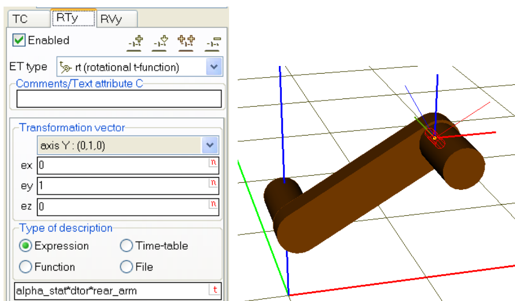
Figure 1.17. Second ET: parameterized rotation
