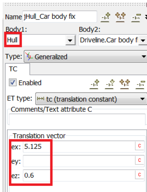
Figure 1.121. Joint connecting fictitious body of transmission with hull
