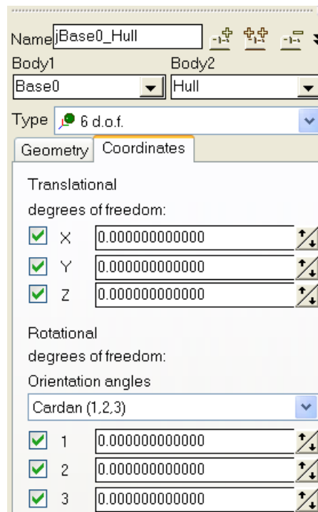
Figure 1.99. Joint introducing six degrees of freedom of a hull relative to Base0
