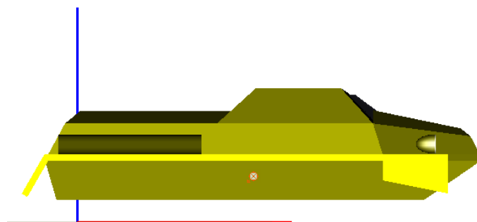
Figure 1.97. Hull-fixed SC coinciding with SC0 for zero values of coordinates
