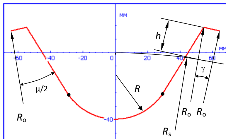
Figure 1.52. Template of sprocket profile for track with one joint a link
