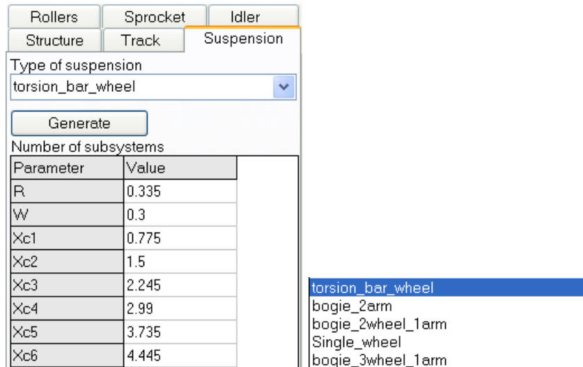
Figure 1.84. Suspension parameters
