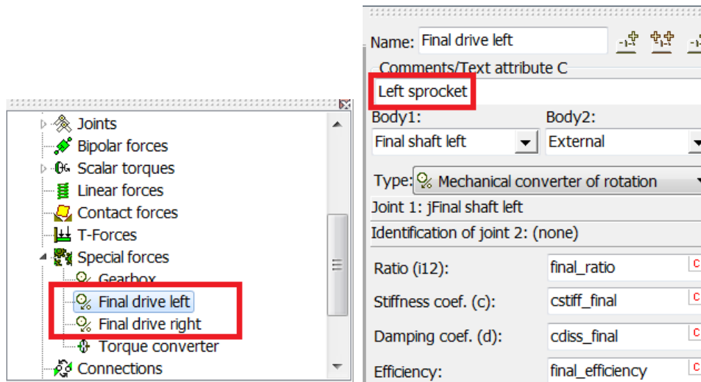
Figure 1.119. Left final drive
