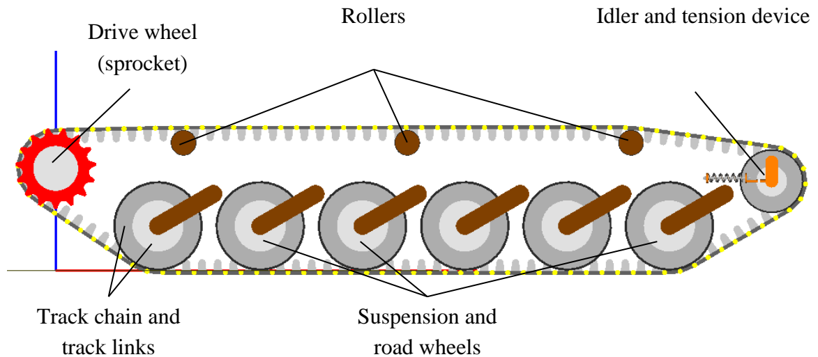
Figure 1.3. Example of a tracked suspension
