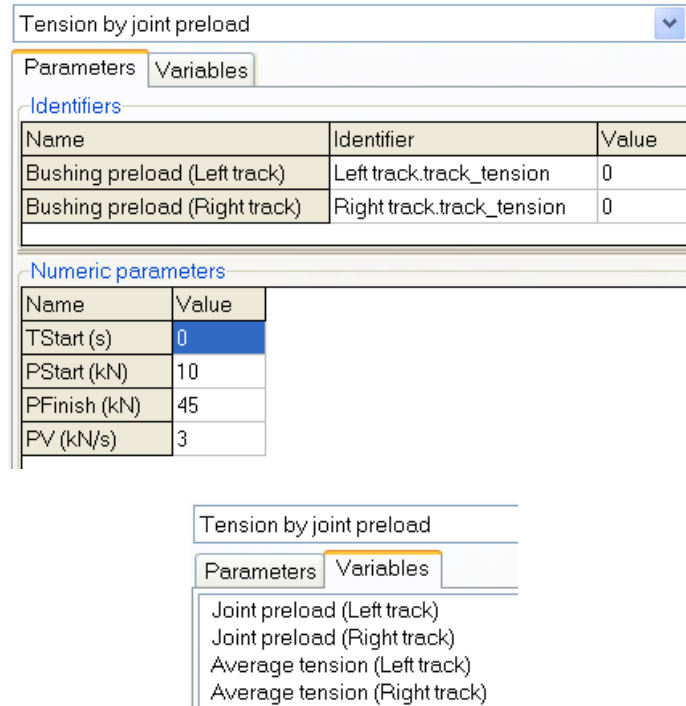
Figure 1.189. Parameters and variables of the test
