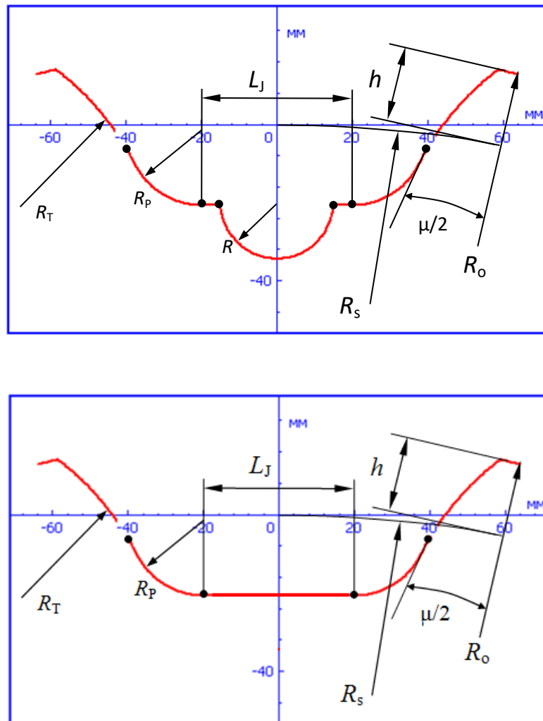
Figure 1.53. Templates of sprocket profile for track with parallel joints
