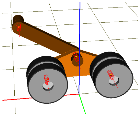
Figure 1.32. Joints
