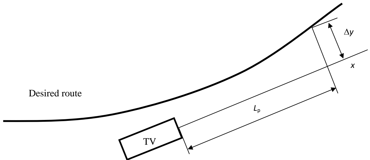
Figure 1.149. To the driver model
