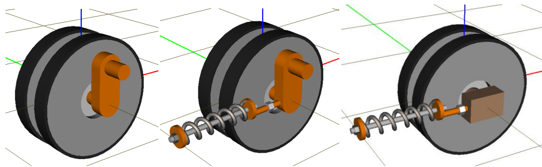
Figure 1.34. Standard models of idler with tension mechanism
