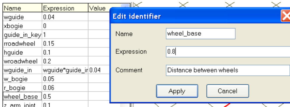
Figure 1.70. Change of bogie base
