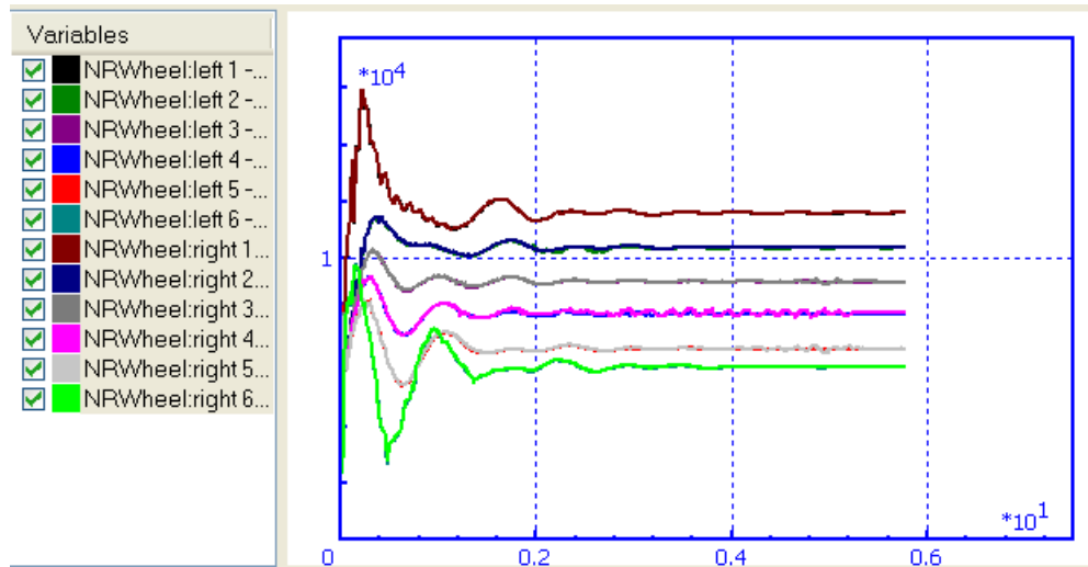
Figure 1.183. Road wheel loads
