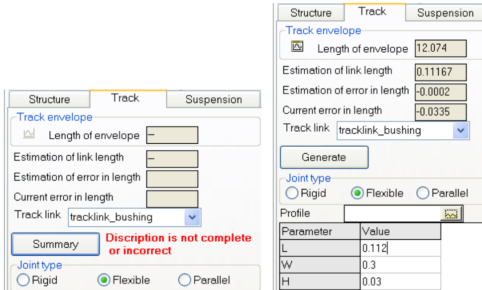
Figure 1.91. Track tab in case of non-complete and complete state
