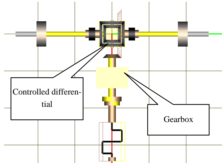
Figure 1.128. Transmission with controlled differential steering
