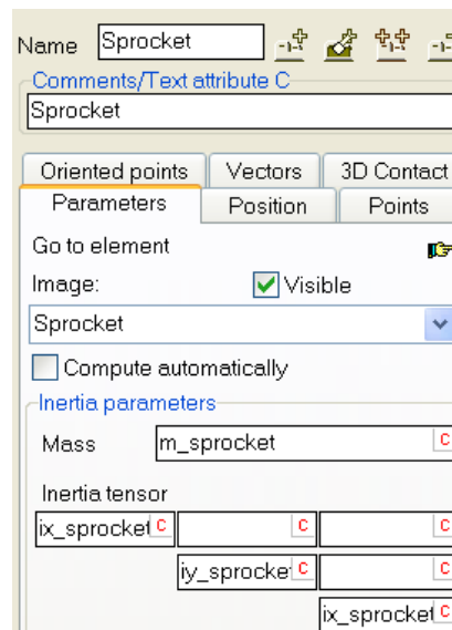
Figure 1.59. Body Sprocket
