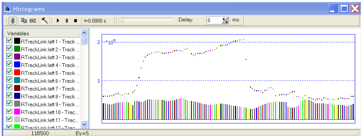
Figure 1.207. Histogram window
