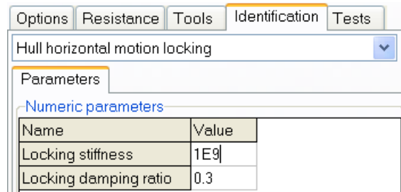
Figure 1.176. Hull locking
