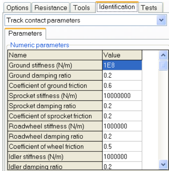
Figure 1.175. Identification of TV model parameters
