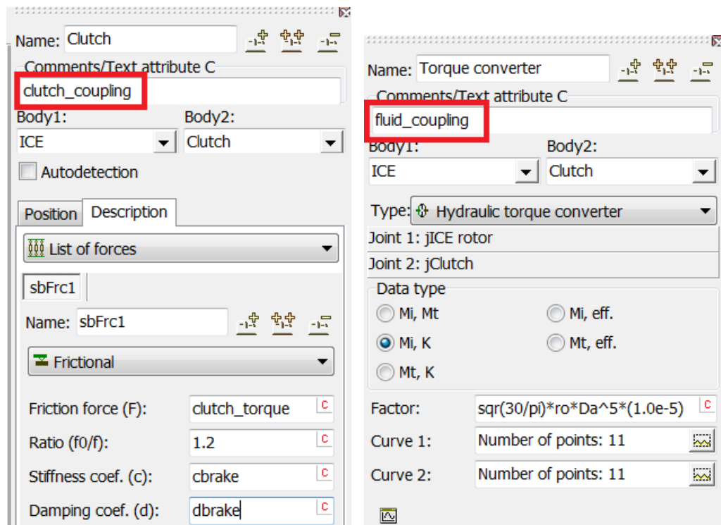
Figure 1.115. Models of clutch and torque converter
