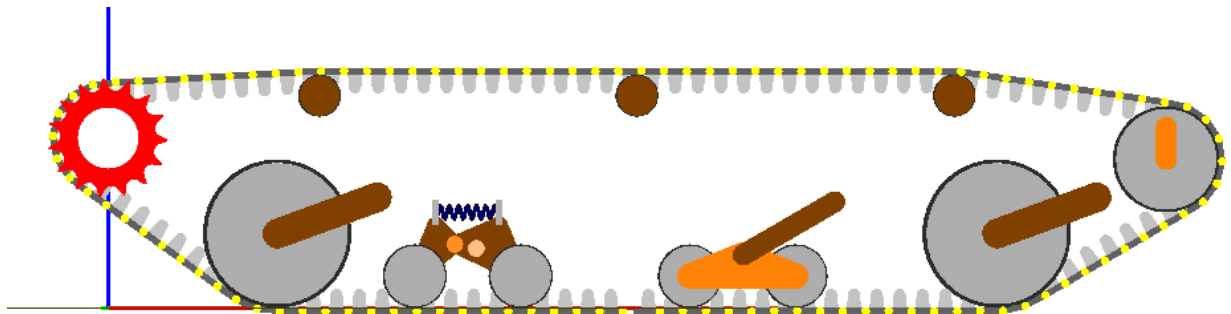
Figure 1.81. Example of a track with three different types of suspensions (for illustration of possibilities only)
