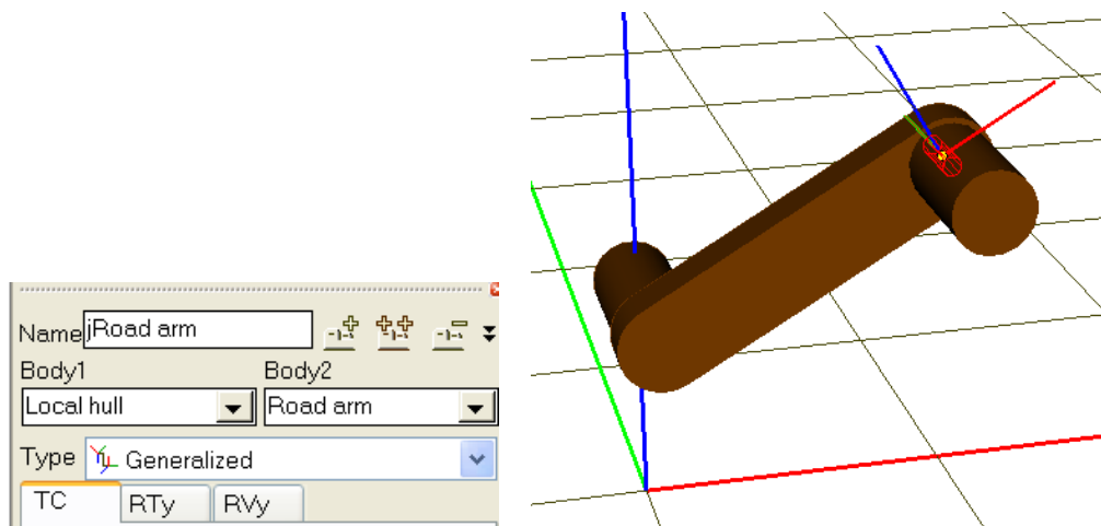
Figure 1.15. Joint jRoad arm and body-fixed SC
