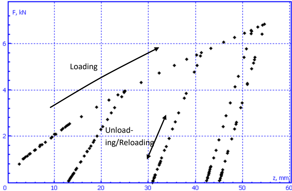
Figure 1.143. Example of track load force versus sinkage by loading and unloading/reloading processes
