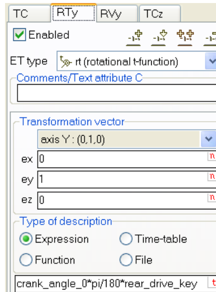
Figure 1.40. The second ET: rotation on a parameterized angle
