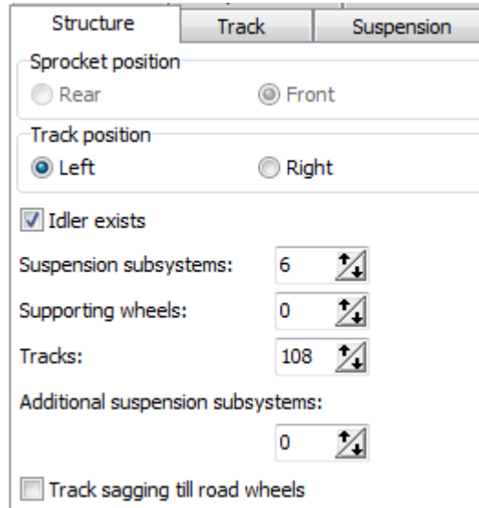
Figure 1.80. Parameters of track structure
