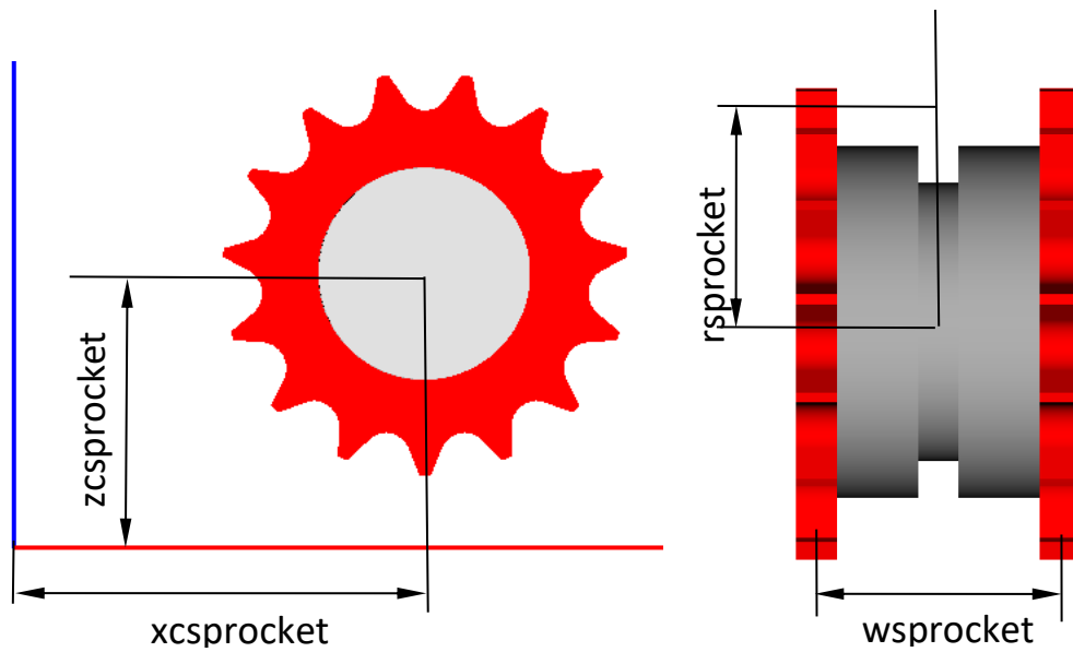
Figure 1.58. Identifiers for geometric parameters of sprocket
