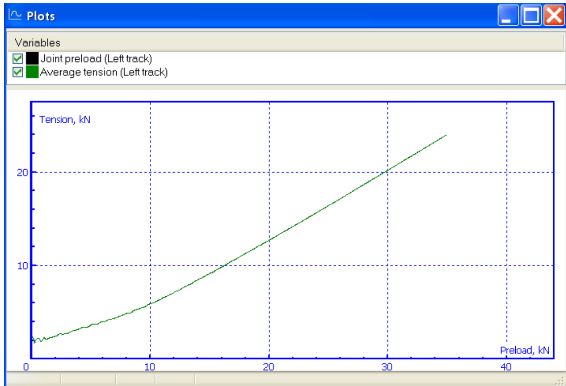
Figure 1.191. Example: tension vs. preload
