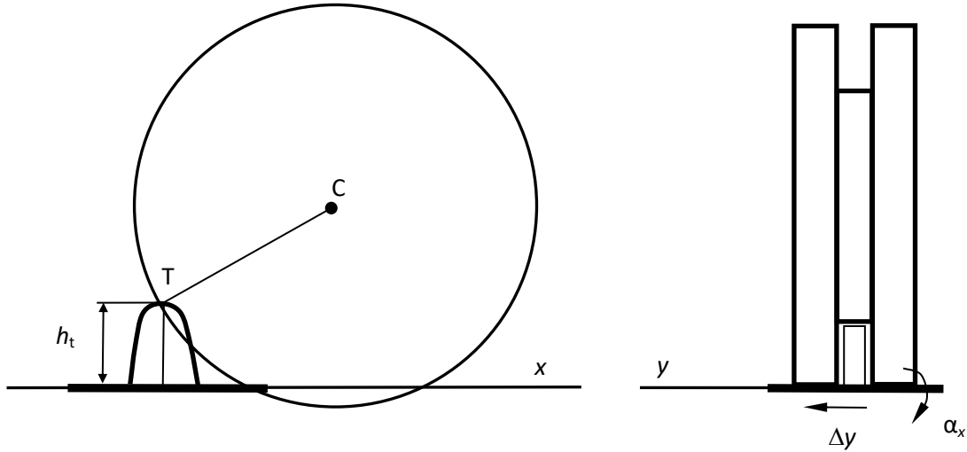
Figure 1.148. Scheme for evaluation of restrictive force and moment
