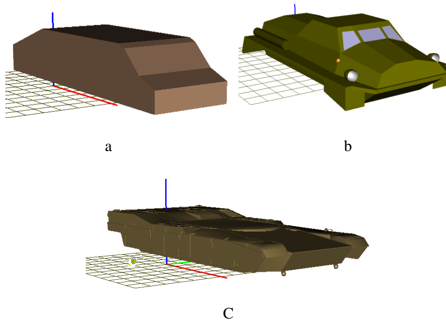
Figure 1.96. Schematic (a), more detailed (b) and imported from CAD hull images
