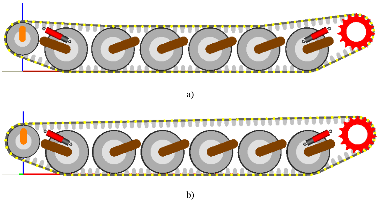
Figure 1.83. Track without supporting wheels with checked (a) and unchecked (b) option 'Track sagging till road wheels'
