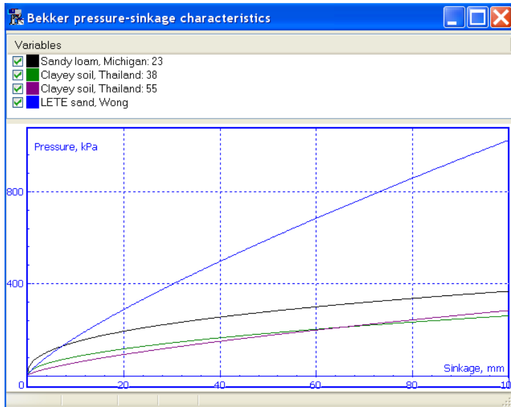
Figure 1.144. Pressure versus sinkage
