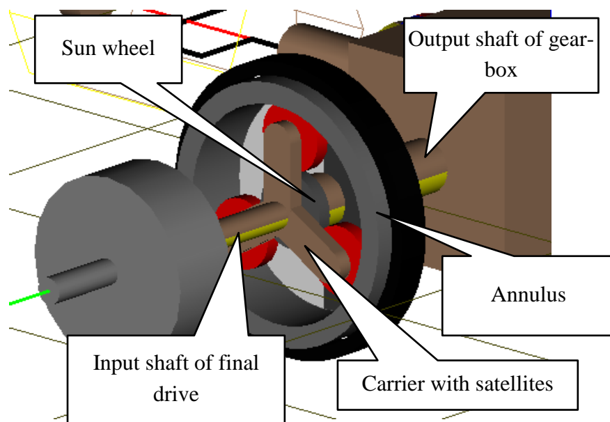
Figure 1.126. Planetary gear
