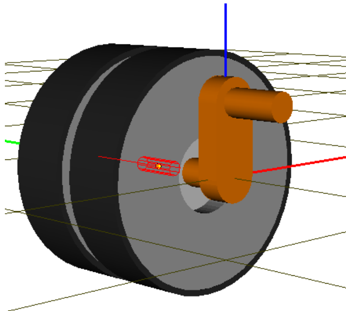
Figure 1.43. Joint jIdler_Tension crank
