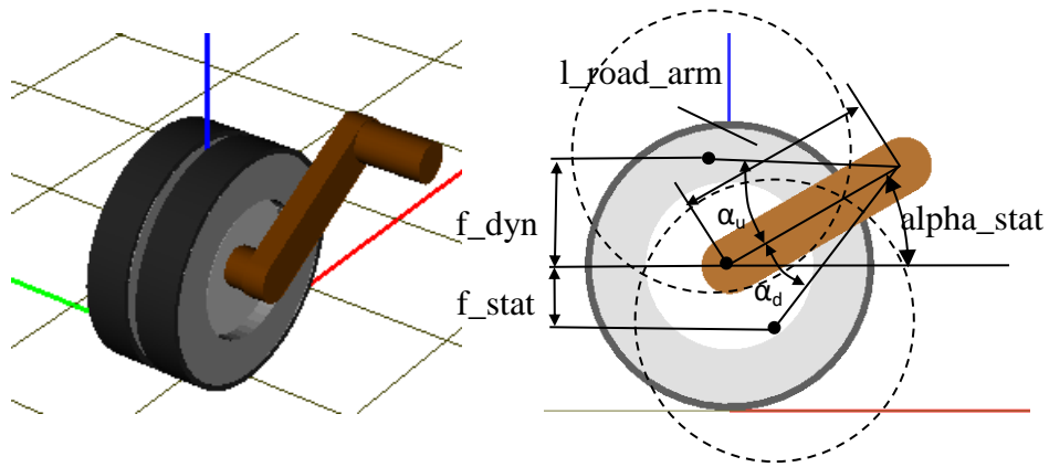
Figure 1.12. Torsion bar suspension and selected identifiers
