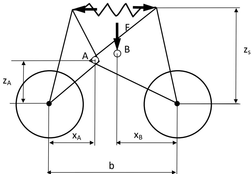
Figure 1.29. Scheme for evaluation of the preload
