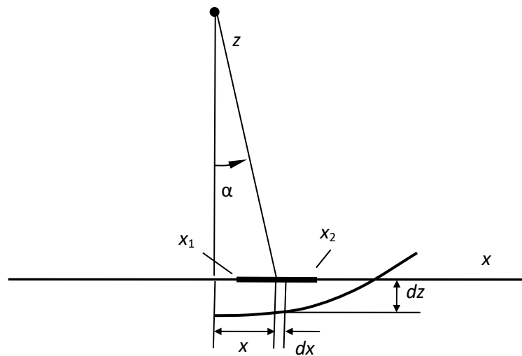
Figure 1.147. Scheme for evaluation of penetration area for a link
