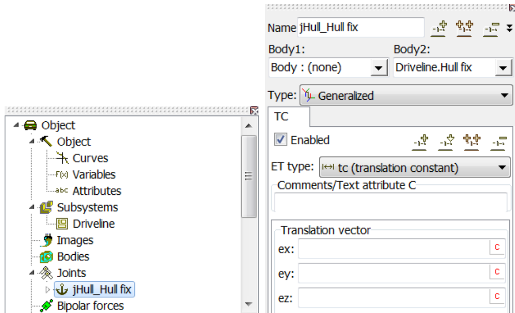
Figure 1.111. Joint for the connection of the fictitious driveline body with the TV hull
