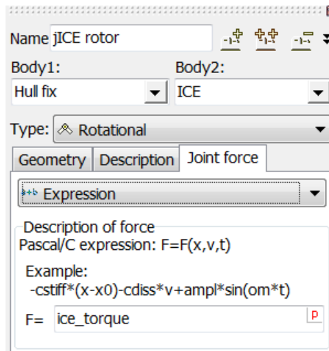
Figure 1.114. Joint specifying rotation of the engine shaft and engine torque
