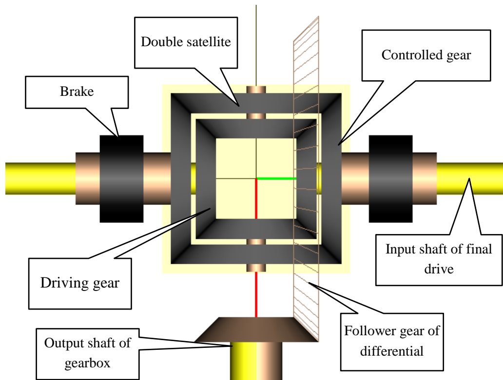
Figure 1.129. Controlled differential
