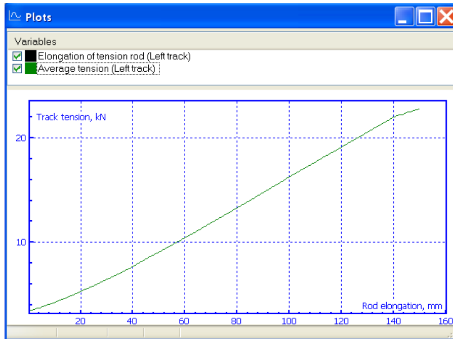
Figure 1.187. Tension vs. elongation
