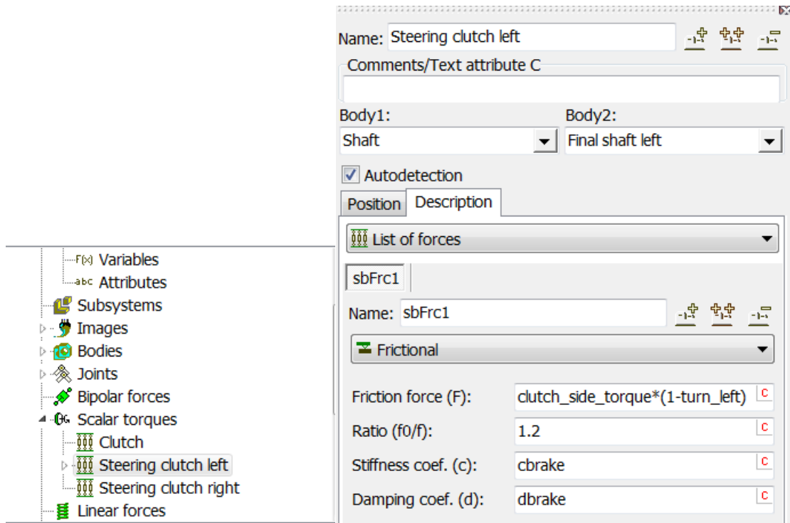
Figure 1.124. Steering clutches
