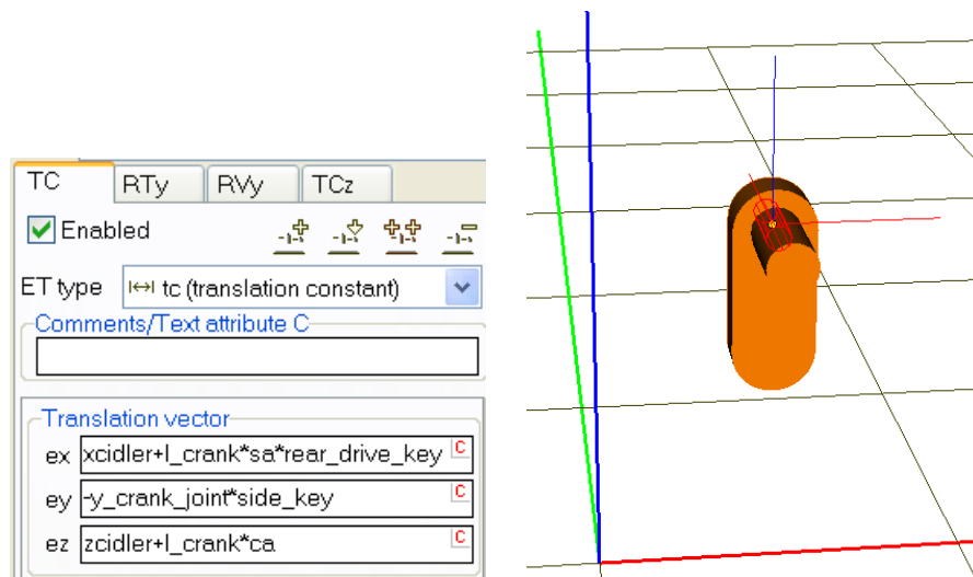
Figure 1.39. The first ET: translation
