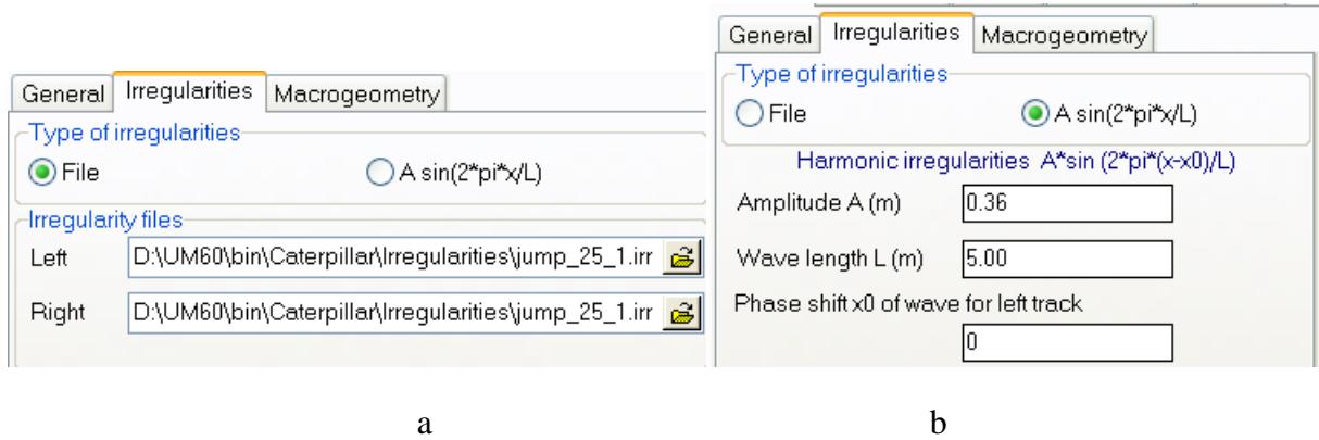
Figure 1.159. File (a) and harmonic (b) irregularities
