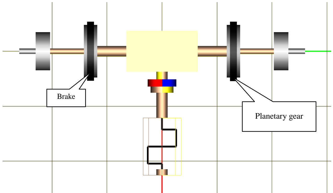
Figure 1.125. Transmission and planetary gear steering system
