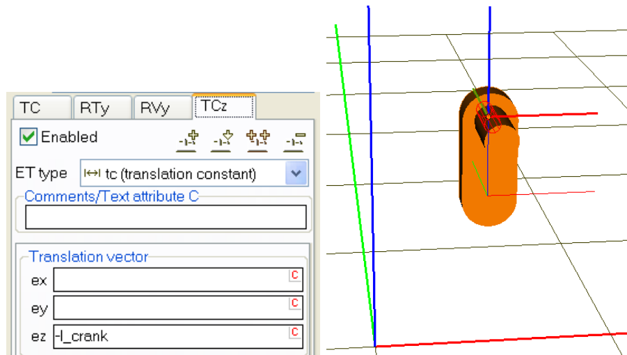
Figure 1.42. The fourth ET: shift to the crank-fixed SC (thick lines)
