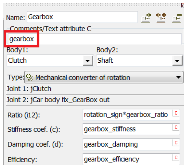
Figure 1.117. Gearbox as a force element
