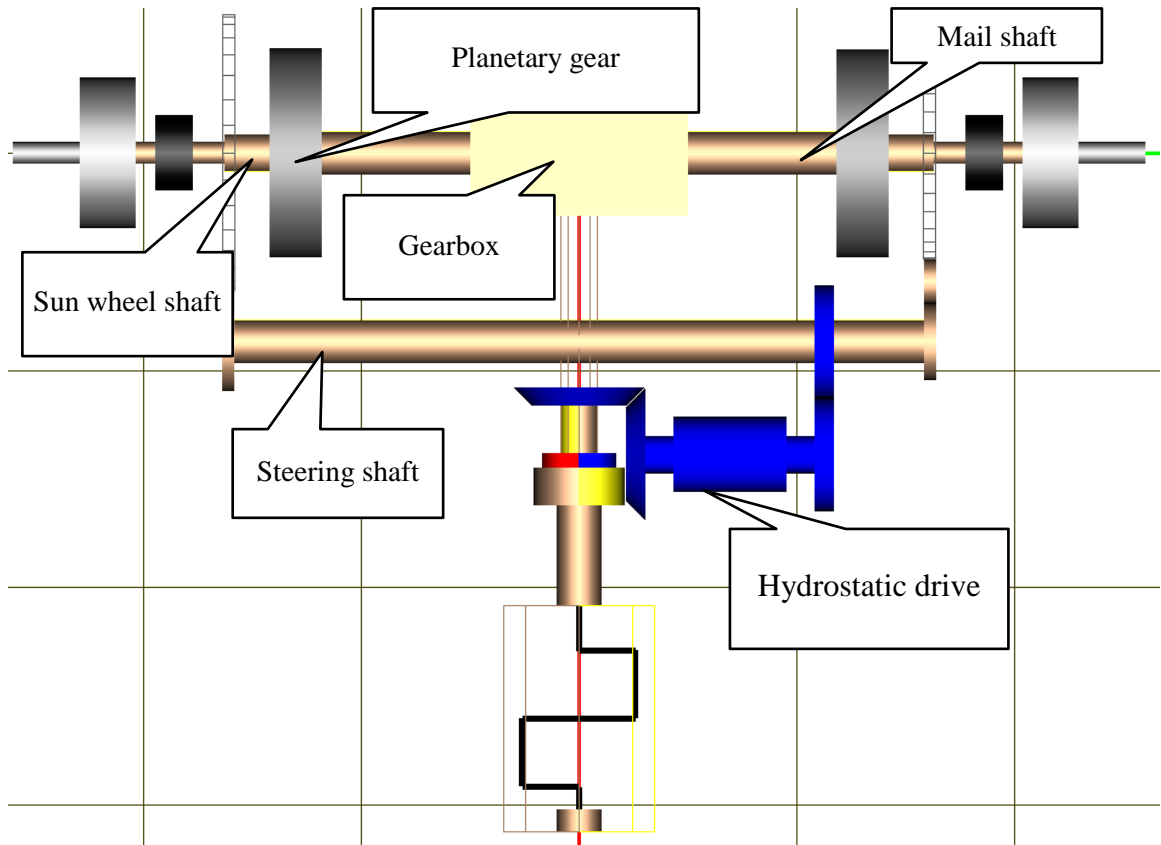
Figure 1.138. Double differential steering system with HSD
