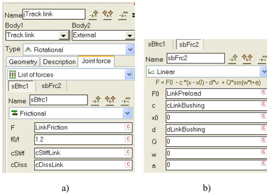
Figure 1.63. Joint torque
