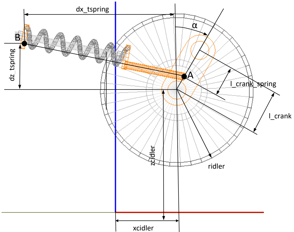
Figure 1.48. Parameterization of model geometry
