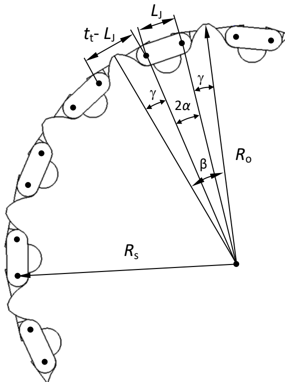
Figure 1.51. Parameters of a sprocket for a track with parallel joints
