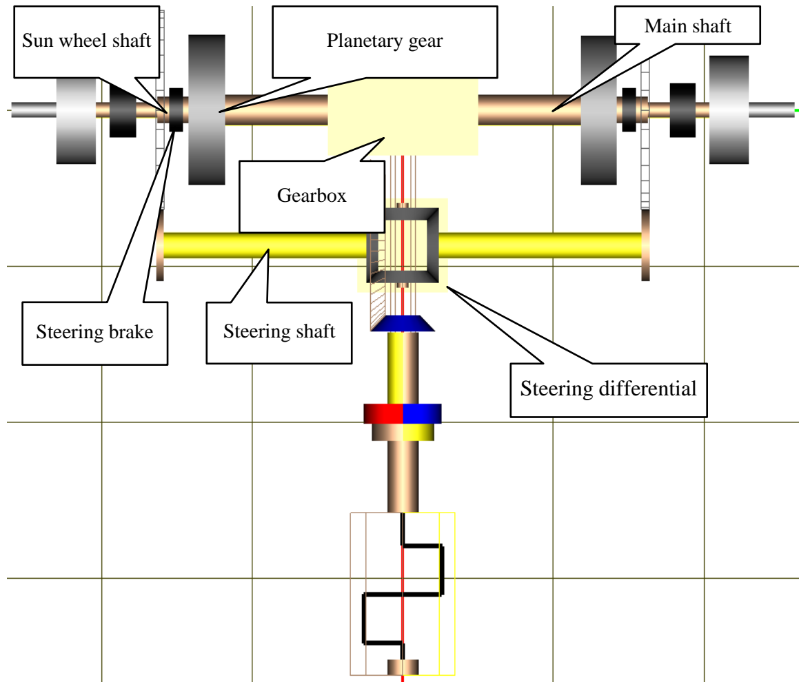
Figure 1.137. Triple differential steering system
