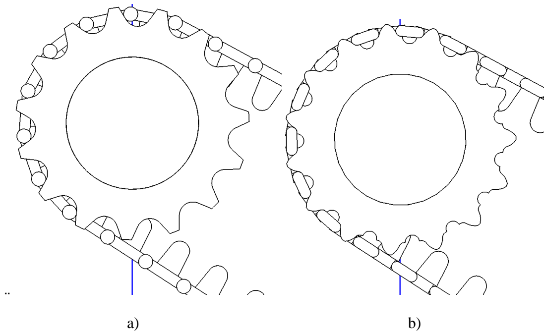
Figure 1.49. Fragments of track models: track links with one joint (a) and with parallel joints (b)
