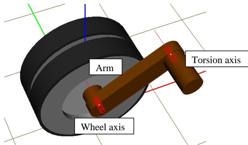
Figure 1.14. Joints in the model of torsion bar suspension
