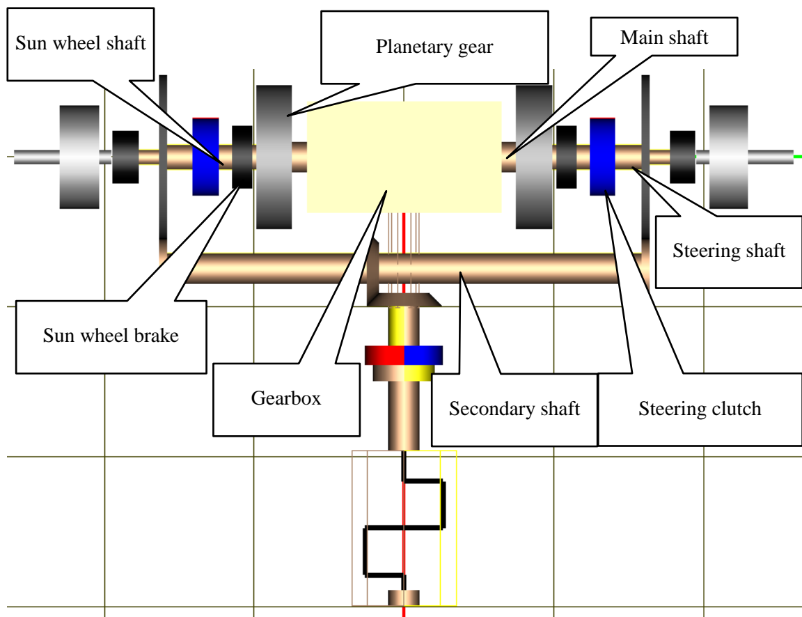
Figure 1.133. "Maybach" double differential steering system
