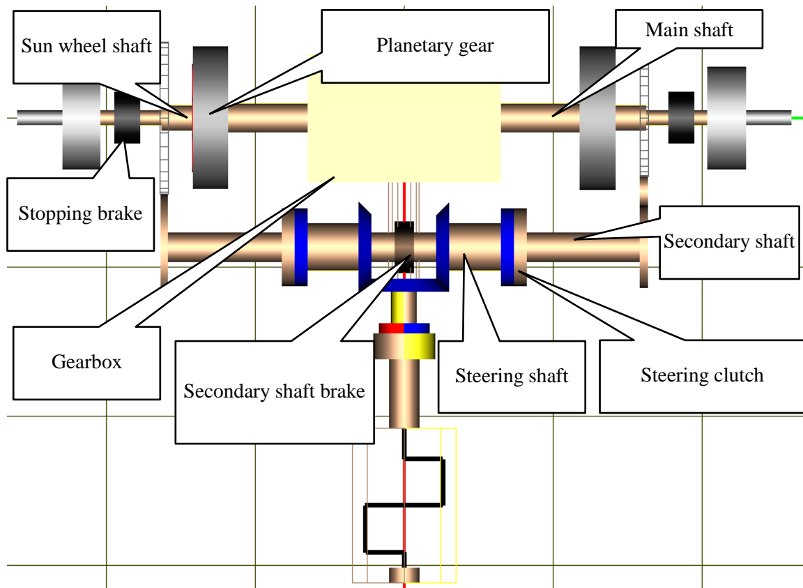
Figure 1.134. Double differential steering system
