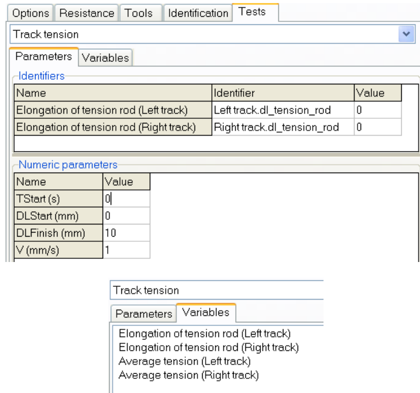
Figure 1.185. Parameters and variables of the test Track tension
