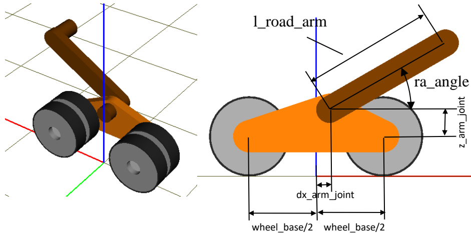
Figure 1.30. Bogie with the torsion-bar (left); selected identifiers (right)
