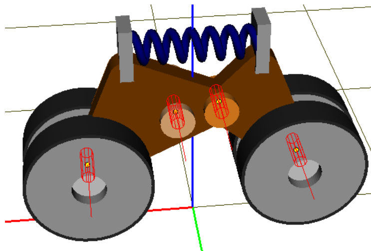
Figure 1.27. Joint of bogie with two arms
