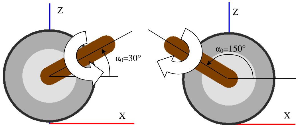
Figure 1.20. Static torques
