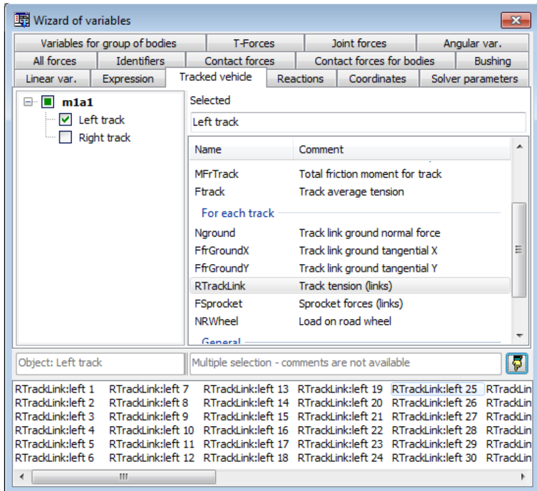
Figure 1.206. List of special TV variables
