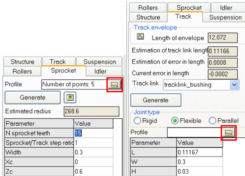
Figure 1.56. Creation and modification of sprocket and pin profiles
