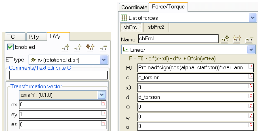
Figure 1.18. Third ET: introduction of rotational degree of freedom and joint torque
