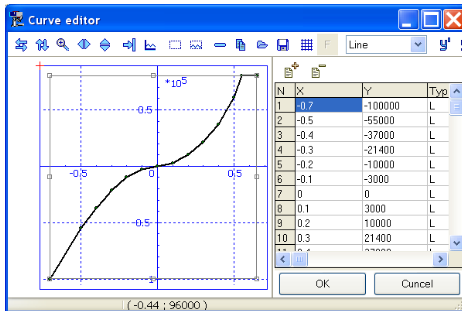
Figure 1.95. Damper as a bipolar force element
