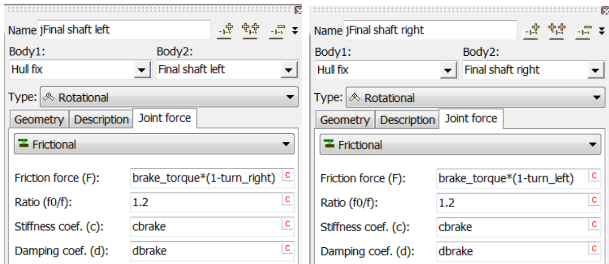
Figure 1.118. Brake torques
