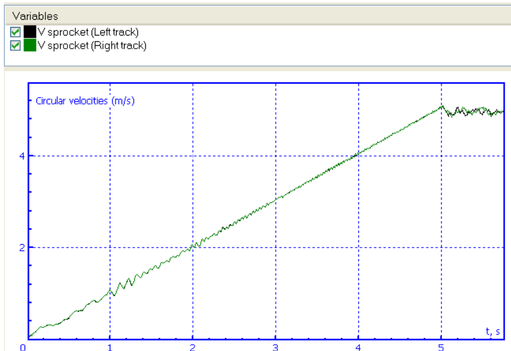
Figure 1.196. Example: circular velocities vs. time
