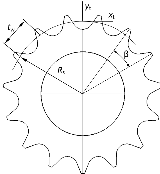
Figure 1.50. Parameters of a sprocket for a track with one joint in a link
