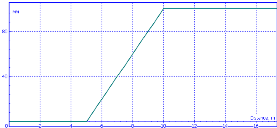
Figure 1.160. Smoothed ground profile
