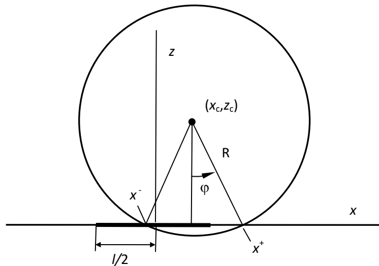
Figure 1.146. Interpenetration of a track link and the wheel
