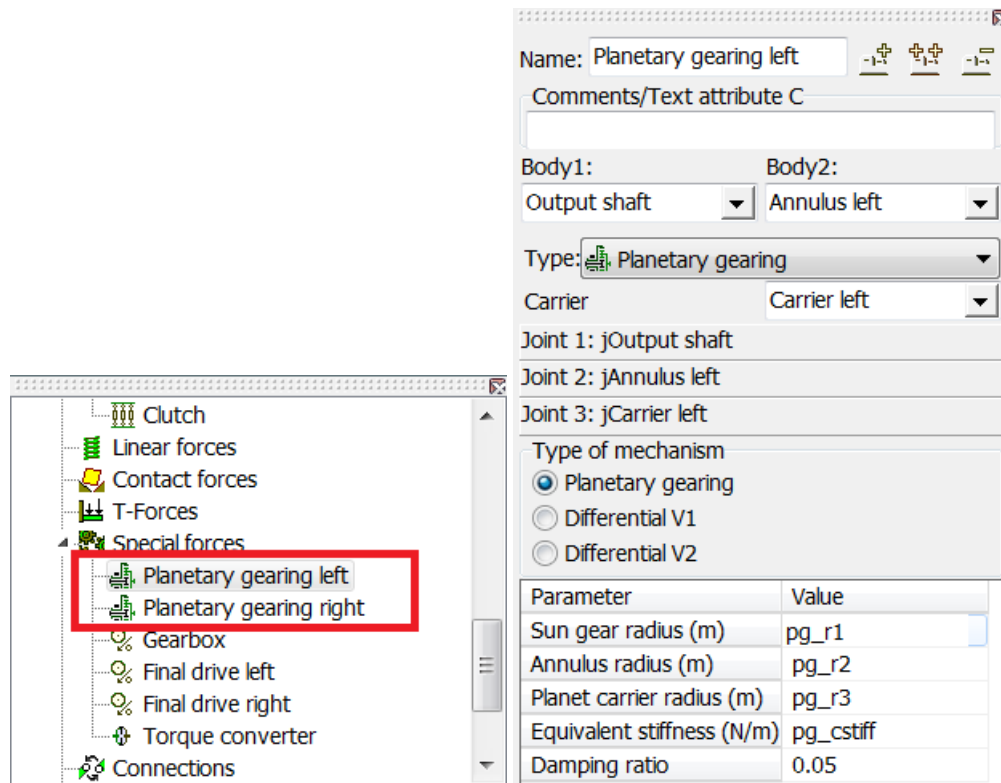
Figure 1.127. Model of planetary gearing
