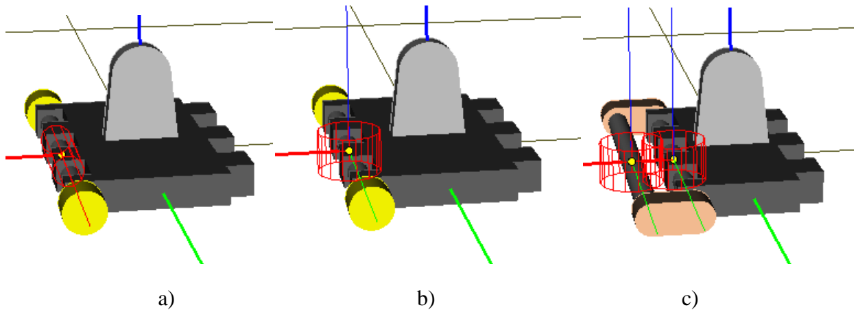
Figure 1.60. Standard models of track links
