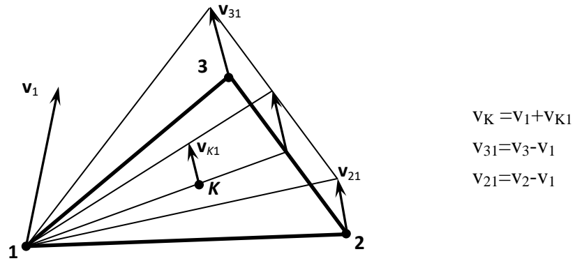
Figure 1.4. On calculation of velocity of an arbitrary point.
