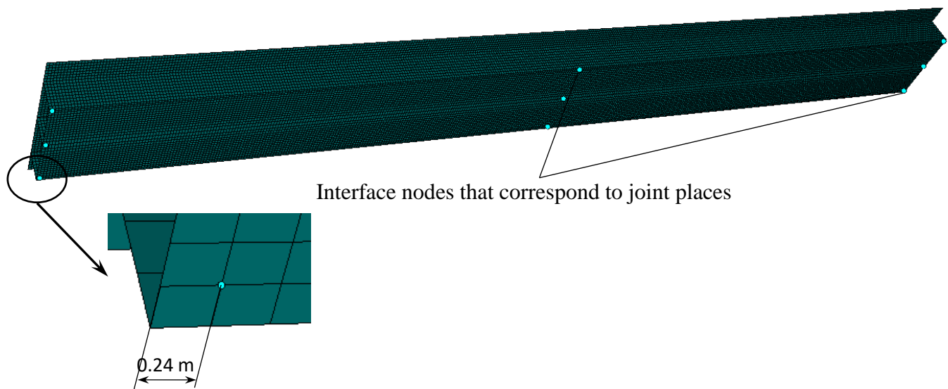
Figure 1.7. Interface nodes of flexible subsystem Bridge.
