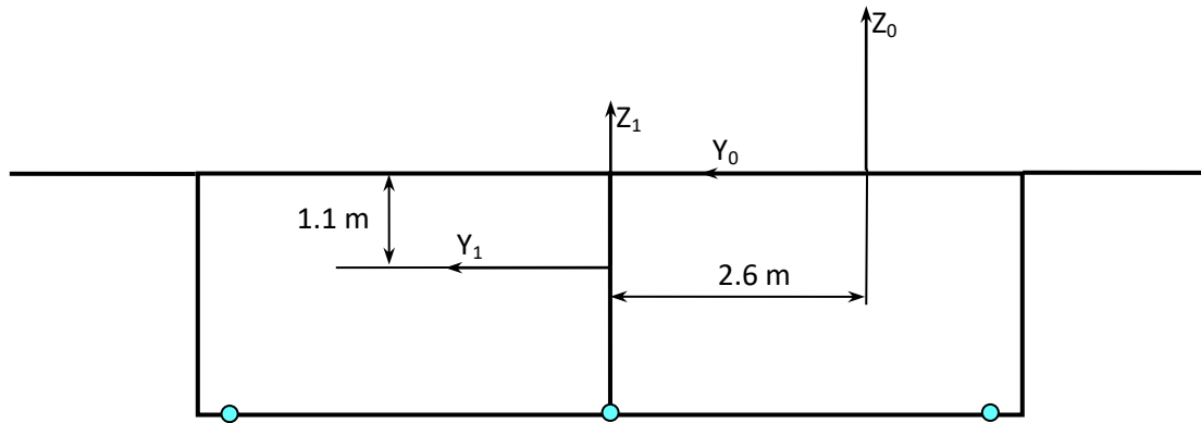
Figure 1.10. Bridge cross section and position of the local frame of reference.
