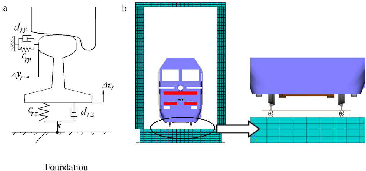
Figure 1.1. (a) rail as a massless force element; (b) visco-elastic foundation including bridge.
