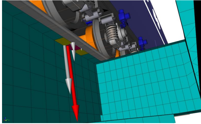
Figure 1.17. Vehicle-bridge interaction force and its reduction to nodal forces.
