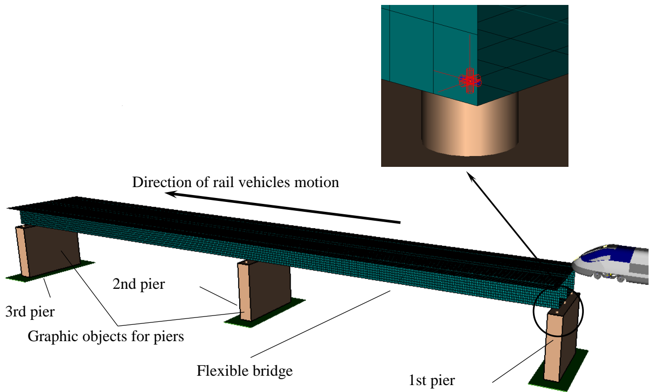
Figure 1.6. Bridge model
