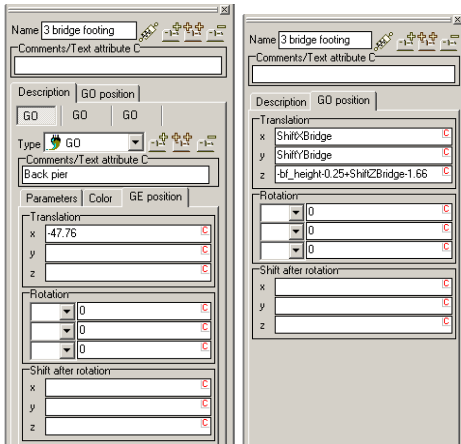
Figure 1.12. Position of the graphical object of the 1st pier (left) and position of 3 bridge footing graphical object assigned to the scene (right).
