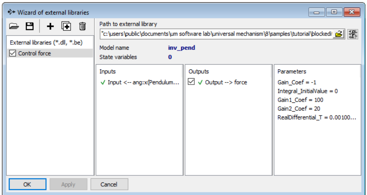
Figure 1.3. Wizard of external libraries
