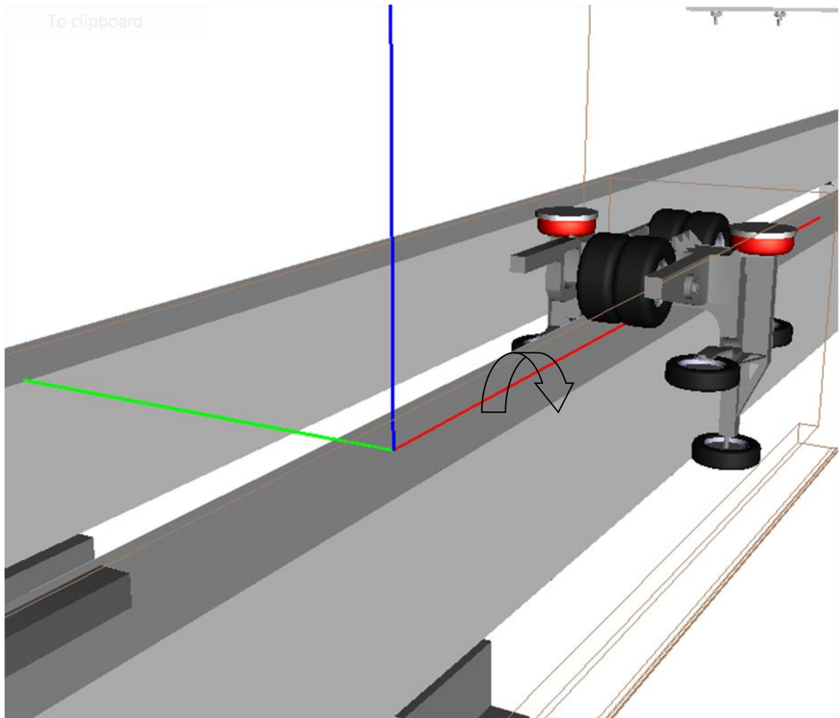
Figure 1.17. Direction of positive superelevation
