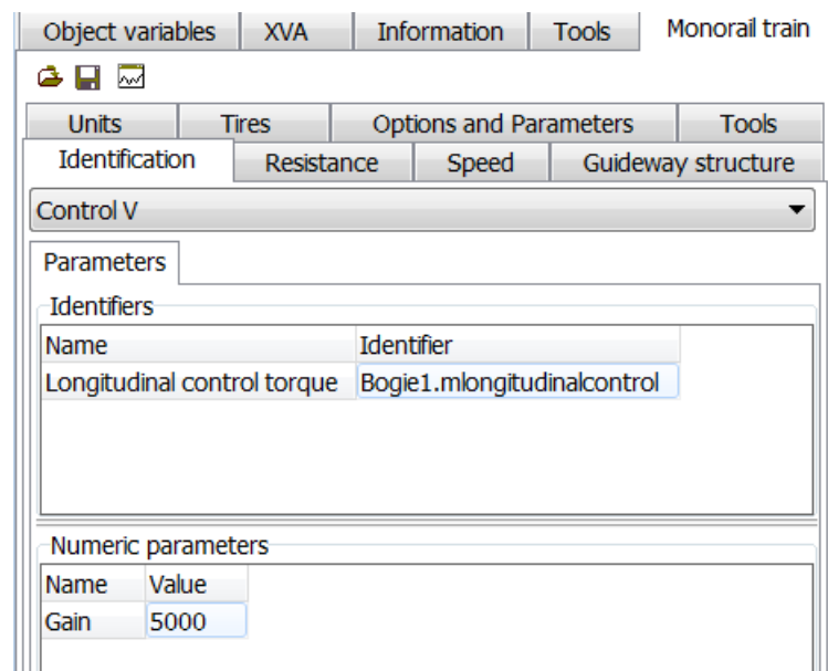
Figure 1.34. Identification of longitudinal velocity control parameters
