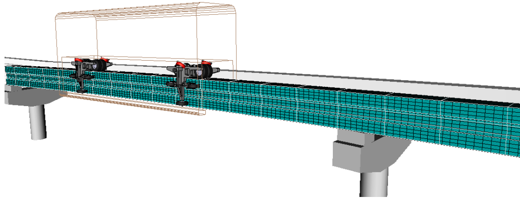
Figure 1.64. Model of supported monorail system from the set of UM samples
