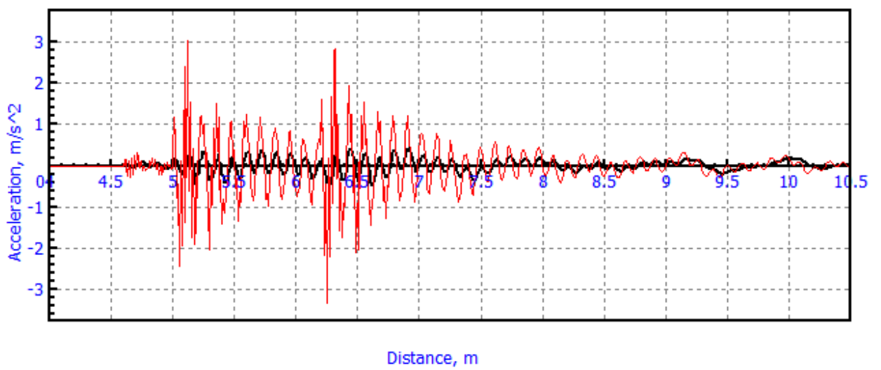
Figure 1.60. Acceleration in the center of track section 30 meters in length. Speed is 5 m/s. Black diagram is obtained with flag Simulation of entry on edge , red is calculated without one.
