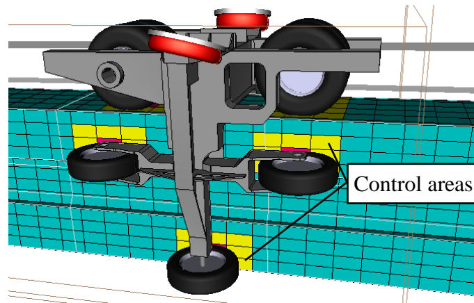
Figure 1.62. Control areas under wheels
