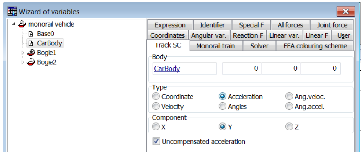
Figure 1.46. Kinematic characteristics of bodies in the track SC
