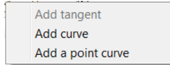
Figure 1.10. Section menu
