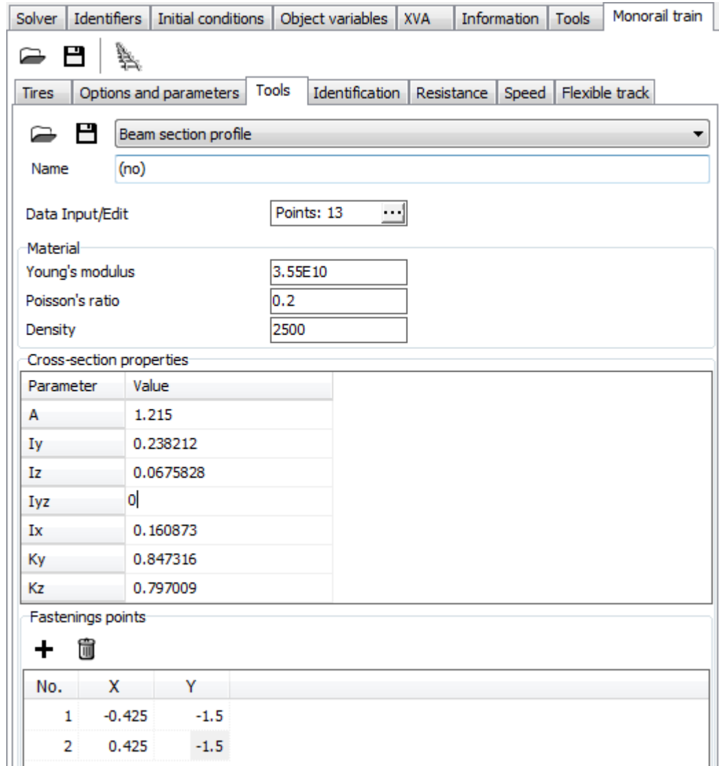
Figure 1.37. Tool for setting beam section
