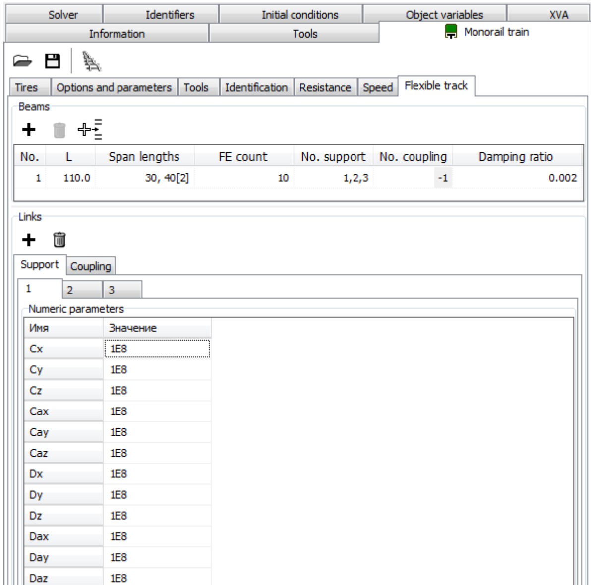
Figure 1.31. Flexible track tab
