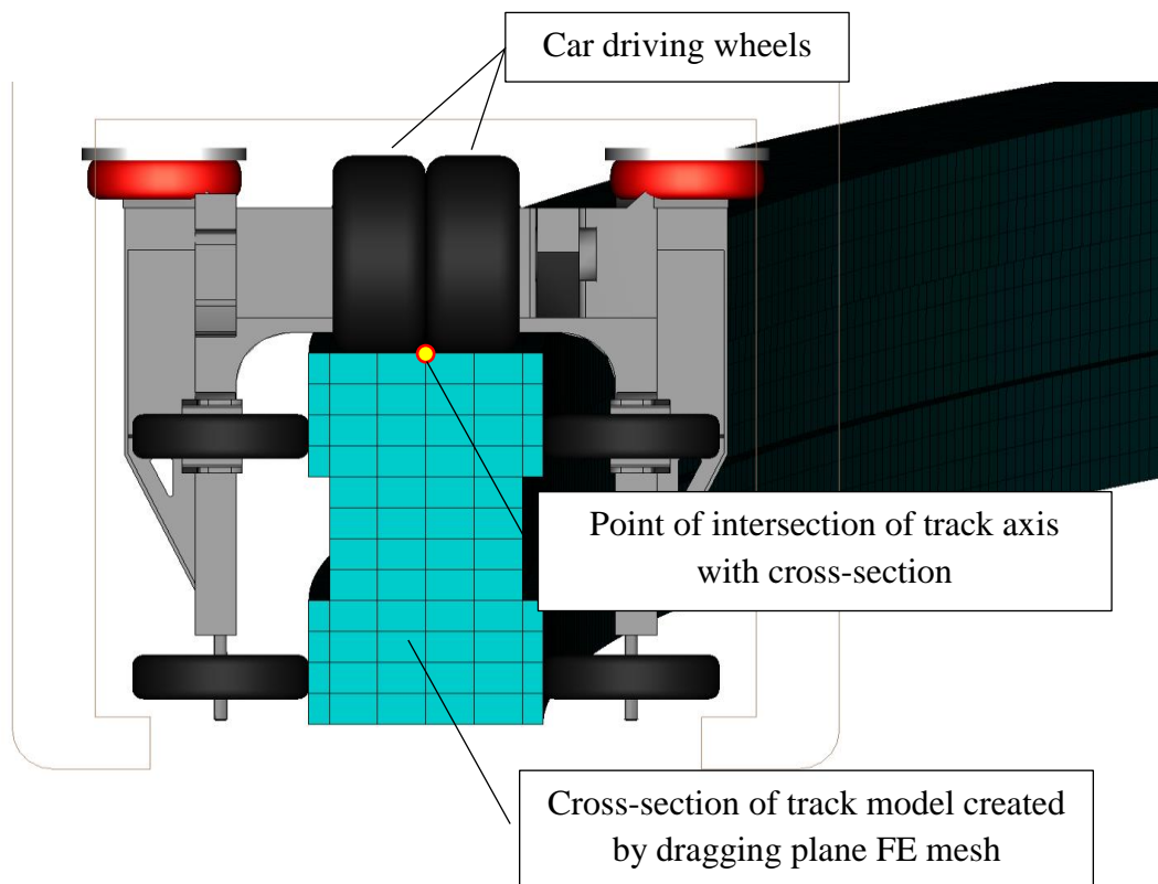
Figure 1.49. Position of the monorail track section relative to the drive wheels
