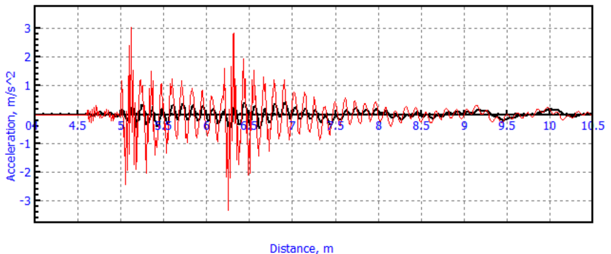
Figure 1.60, the diagram of acceleration in the center of track section 30 meters in length under entry of the vehicle on the edge is shown as example.
