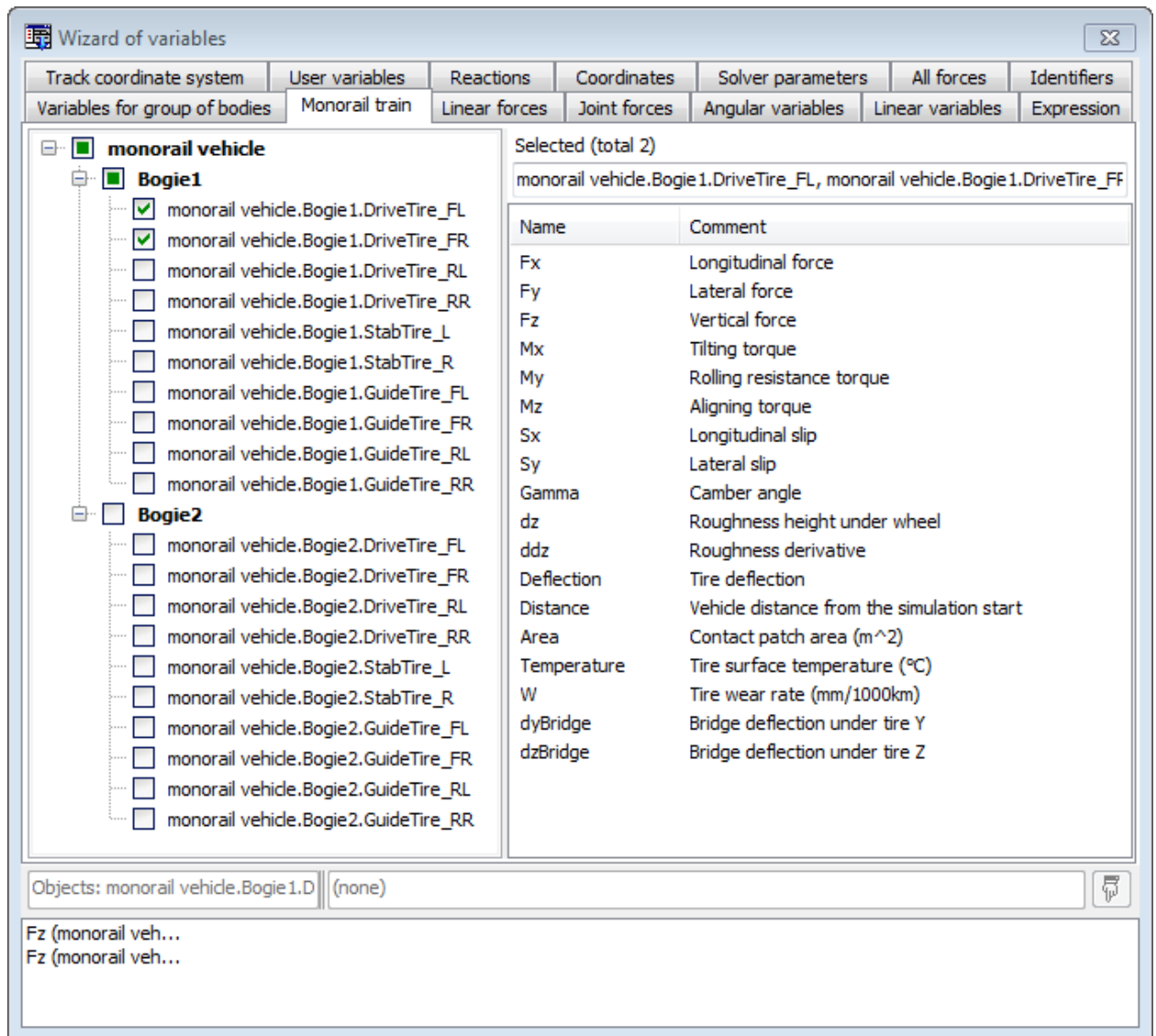
Figure 1.45. Variables related to tire/beam interaction
