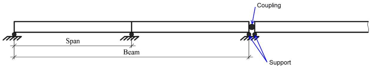
Figure 1.29. Model of a flexible monorail track
