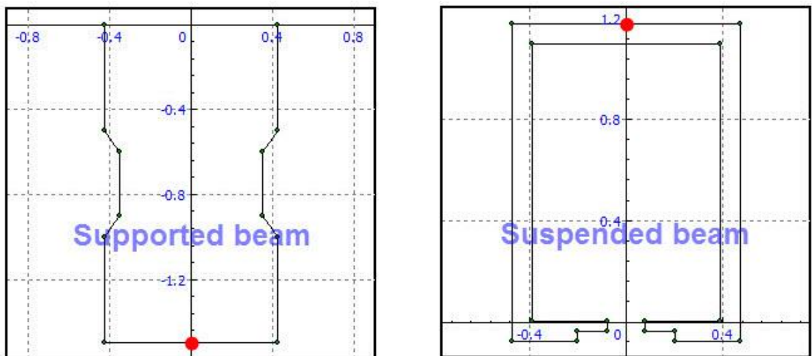
Figure 1.39. Location of default fastening points for different types of monorail beams
