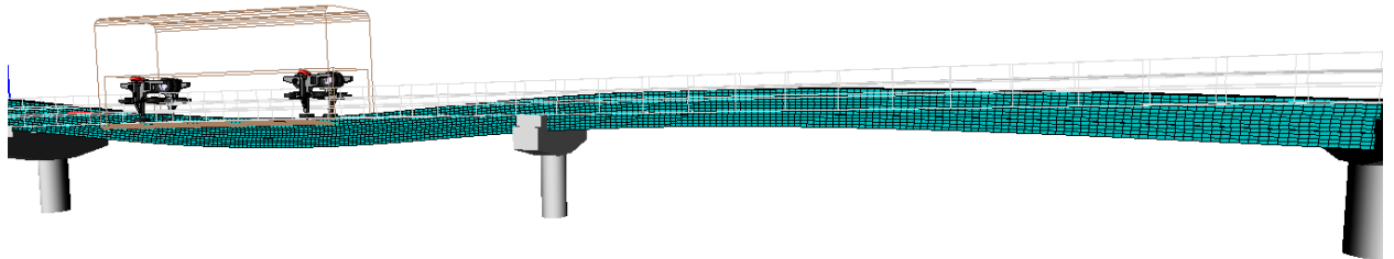
Figure 1.63. Flexible deflections of the monorail track are scaled in 200 times.
