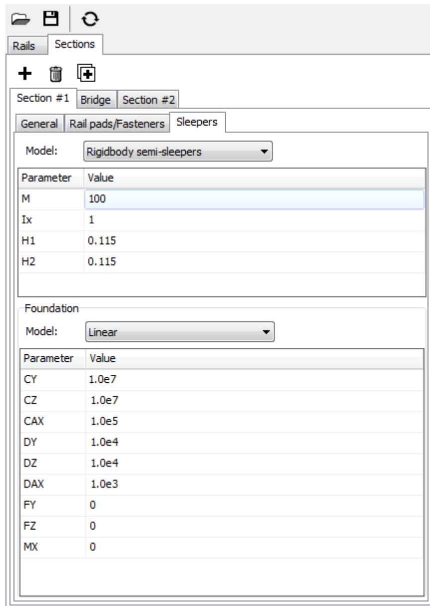
Figure 27.17. Parameters of rigid semi-sleepers
