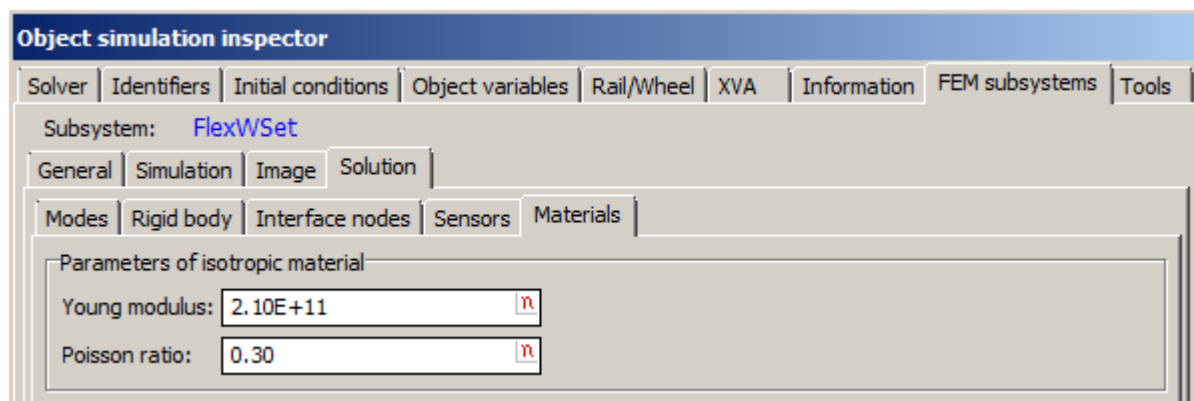
Figure 28.34. Input properties of wheelset material
